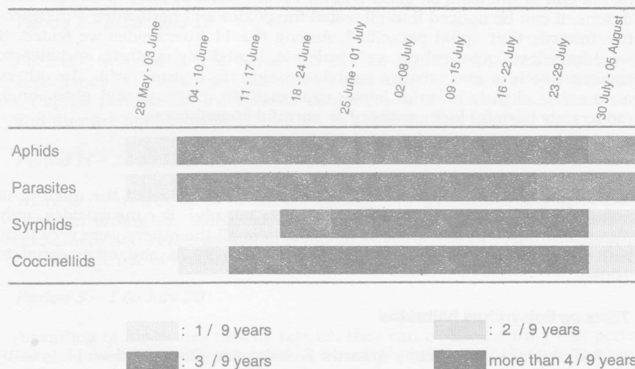
Figure 1. Appearance frequency of aphids and aphidophagous in Belgian potato crops between 1994 and 2002.
