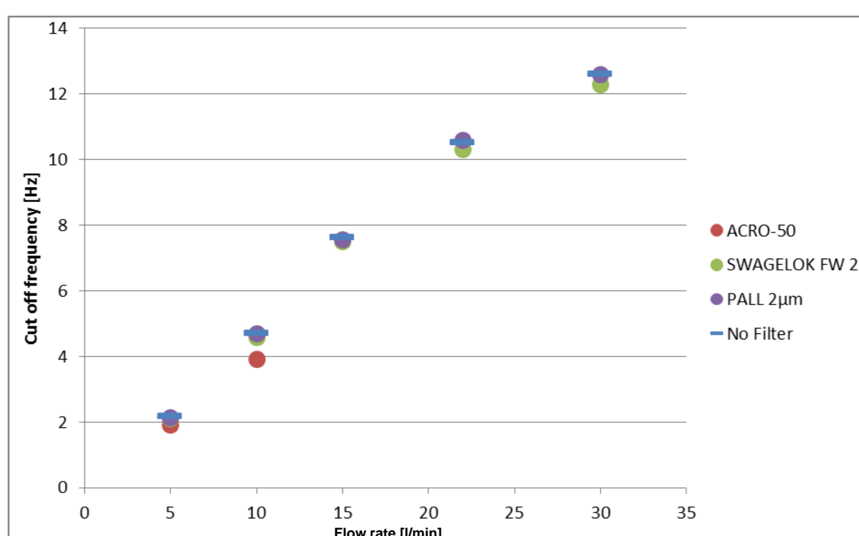
Fig 3: Cut-off frequencies (Hz) in function of the flow rate (l/min) for LI-7200 with ACRO-50 (red), Pall 2 \mu m (purple), Swagelok FW 2 \mu m (green), and without any filter (blue)
