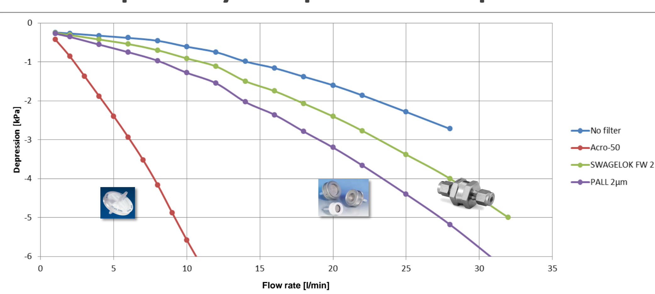
Fig 2: Depression in IRGA cell (kPa) in function of the flow rate (l/min) for LI-7200 with ACRO-50 (red), Pall 2 \mu m (purple), Swagelok FW 2 \mu m (green), and without any filter (blue)
