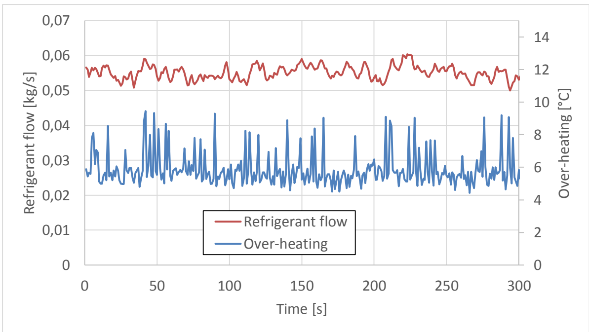
Figure 28: Oscillations of the flow due to the electronic expansion valve due to low set-point of over-heating
