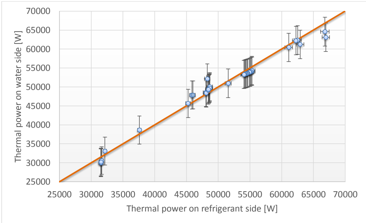
Figure 25: Evaporator heat balance (ORC)
