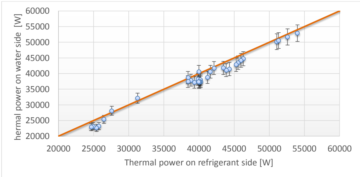
Figure 23: Heat balance on the condenser (ORC).
