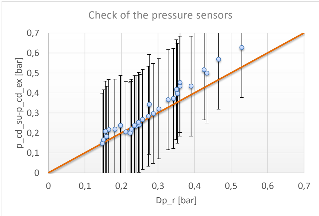
Figure 21: Cross-checking of pressure sensor of the condenser (ORC)
