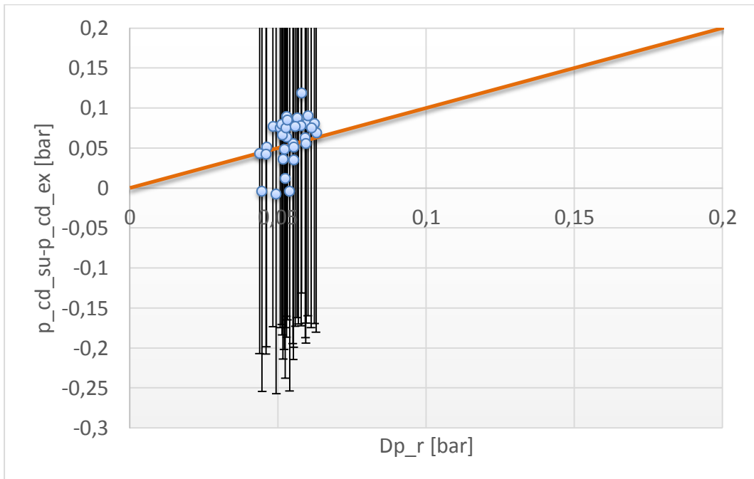
Figure 20: Cross-checking of pressure sensor of the condenser (Heat pump)
