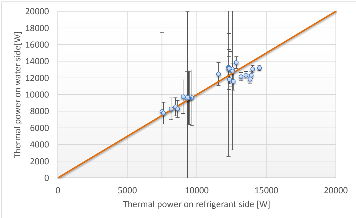
Figure 24: Evaporator heat balance (heat pump)
