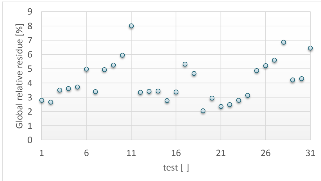
Figure 18: Global relative residue (heat pump)
