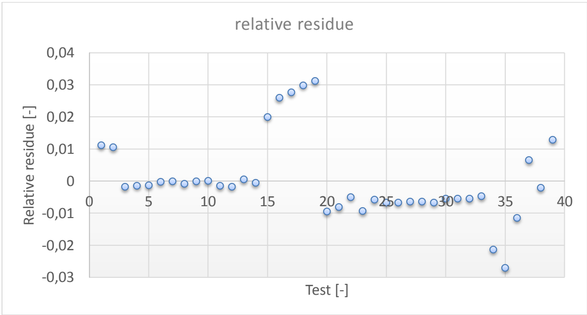
Figure 19: Global relative residue (ORC)
