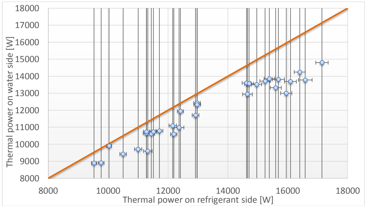
Figure 22: Heat balance on the condenser (heat pump)
