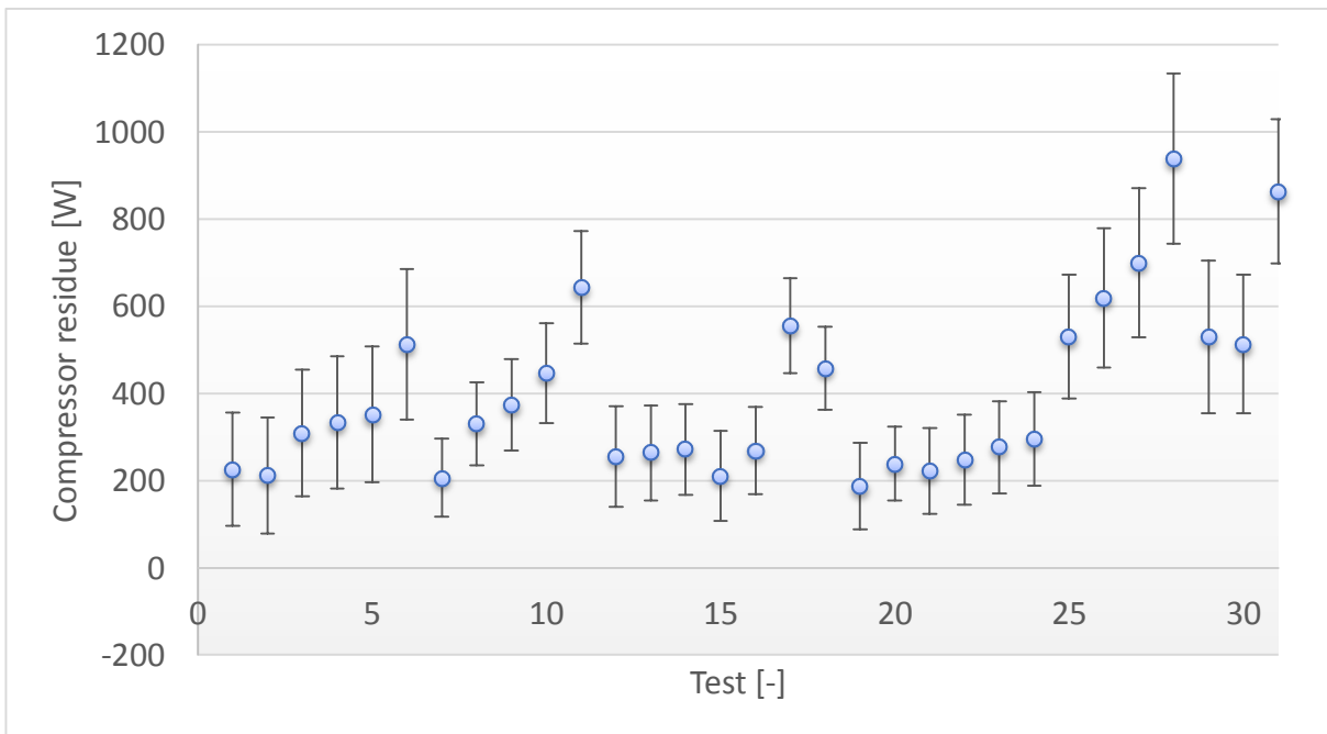
Figure 26: Compressor residue
