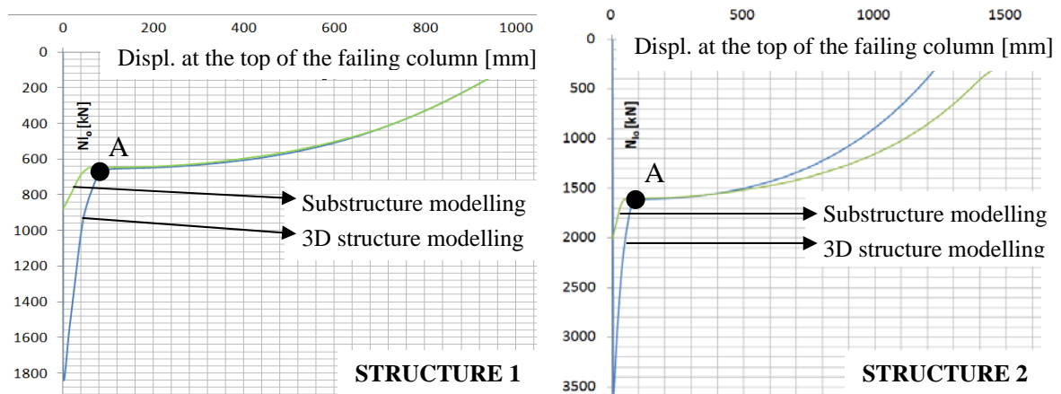
Fig. 10: Comparisons between the results obtained through numerical simulations (i) of the 3D structure and (ii) of the substructure
