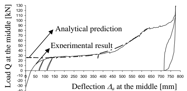
Fig. 7: Comparison analytical prediction vs. experimental results
