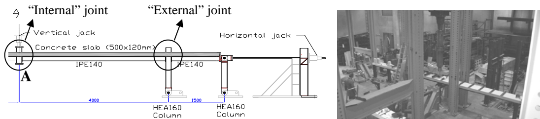
Fig. 4: Tested substructure
