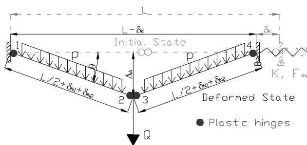
Fig. 6: Substructure to be investigated
