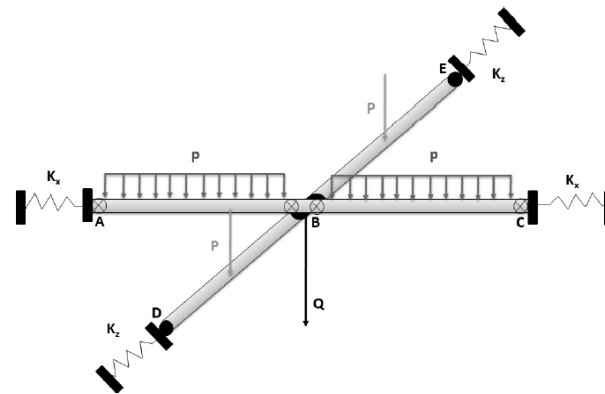
Fig. 9: Substructure extracted from the 3D structure
