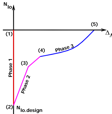
Fig. 2: Evolution of N_{Io} according to the vertical displacement at the top of the lost column
