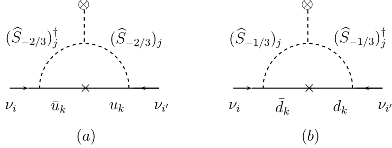
Figure 1: Feynman diagrams for Majorana neutrino masses. Diagram (a) [(b)] give contributions to the neutrino mass matrix from u -type [ d -type] quarks loops.
