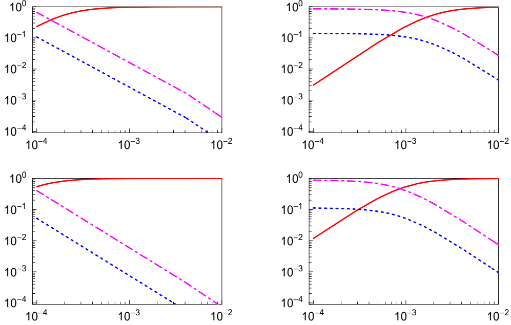
Figure 7: Typical values for decay branching ratios for the heavier Q = 4/3 LQ, in case W^\pm final states are kinematically closed. Branching ratios are plotted versus the “average” Yukawa coupling \bar{\lambda} \equiv \sqrt{\sum_i \lambda_{i3}^2} , for different values of Y_{S_1} and m_2^{Q=4/3} . Full line (red): fermionic final states, dashed line (blue) Higgs final state, dot-dashed (magenta) Z^0 final state. In all figures m_1^{Q=4/3} has been set to m_1^{Q=4/3} = 250 GeV and we have chosen m_{h^0} = 115 GeV, motivated by the LEP limit. Top left: ( Y_{S_1} = 0.01, m_2^{Q=4/3} = 400 GeV); top right: ( Y_{S_1} = 0.1, m_2^{Q=4/3} = 400 GeV); bottom left: ( Y_{S_1} = 0.01, m_2^{Q=4/3} = 800 GeV); bottom right: ( Y_{S_1} = 0.1, m_2^{Q=4/3} = 800 GeV).
