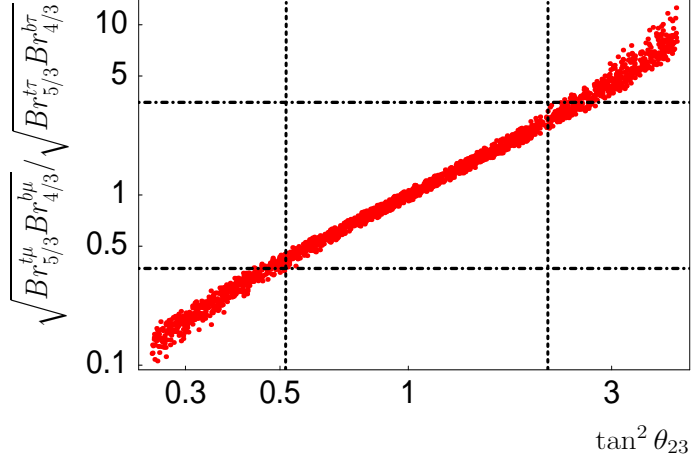
Figure 2: Ratio of decay branching ratios \sqrt{Br_{5/3}^{t\mu} Br_{4/3}^{b\mu}} / \sqrt{Br_{5/3}^{t\tau} Br_{4/3}^{b\tau}} versus \tan^2 \theta_{23} . Vertical lines indicate current 3\sigma range for \tan^2 \theta_{23} while horizontal lines determine the predicted range for this observable.
