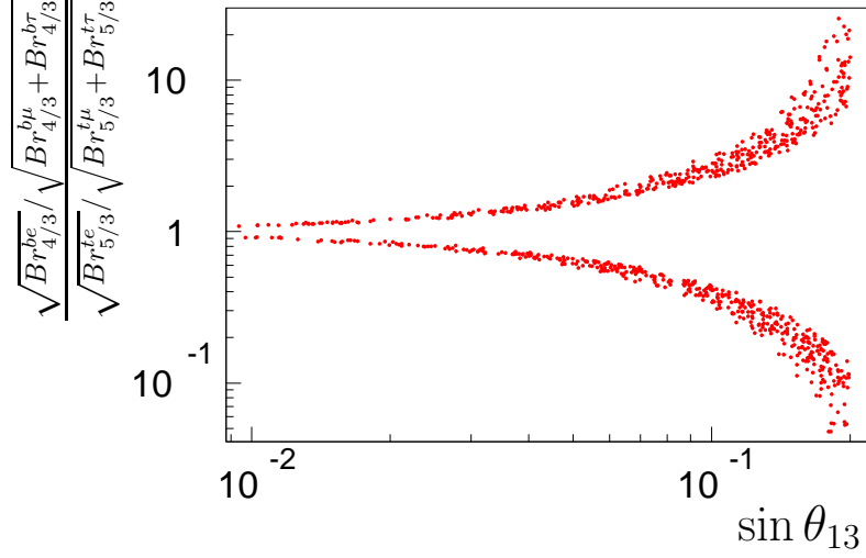
Figure 5: Ratio of decay branching ratios \sqrt{Br_{4/3}^{be}/\sqrt{Br_{4/3}^{b\mu} + Br_{4/3}^{b\tau}}}/\sqrt{Br_{5/3}^{te}/\sqrt{Br_{5/3}^{t\mu} + Br_{5/3}^{t\tau}}} versus \sin \theta_{13} .
