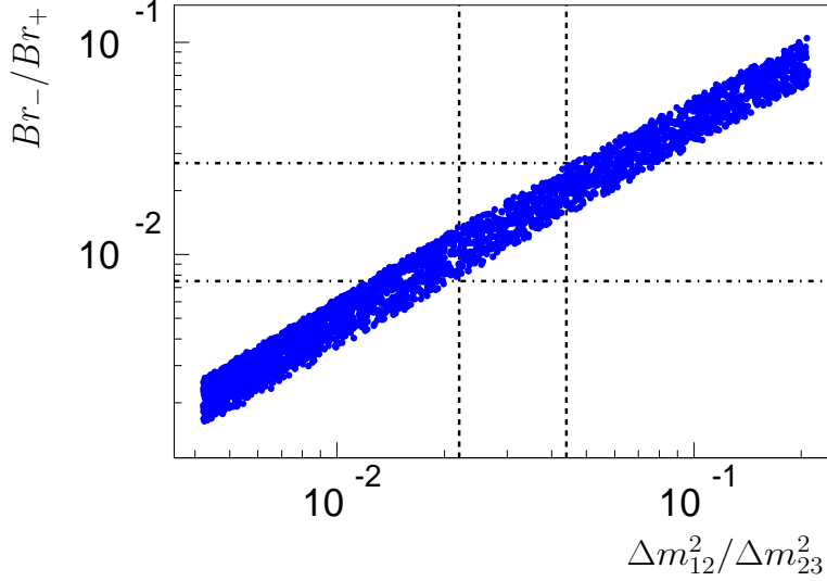
Figure 6: Ratio of decay branching ratio Br_-/Br_+ versus R . Vertical lines indicate current 3\sigma range for R whereas horizontal lines show the predicted range for this observable. The spread of the points in the plot determine the uncertainty with which this ratio can currently be predicted.
