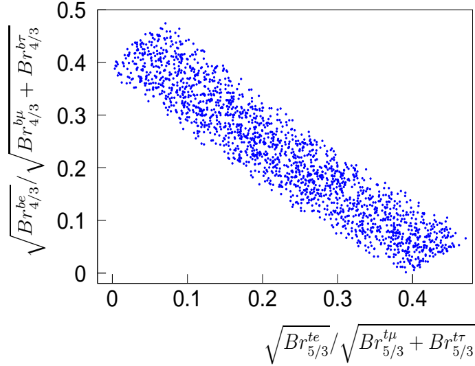
Figure 4: Ratio of decay branching ratios \sqrt{Br_{4/3}^{be}} / \sqrt{Br_{4/3}^{b\mu} + Br_{4/3}^{b\tau}} versus \sqrt{Br_{5/3}^{te}} / \sqrt{Br_{5/3}^{t\mu} + Br_{5/3}^{t\tau}} .
