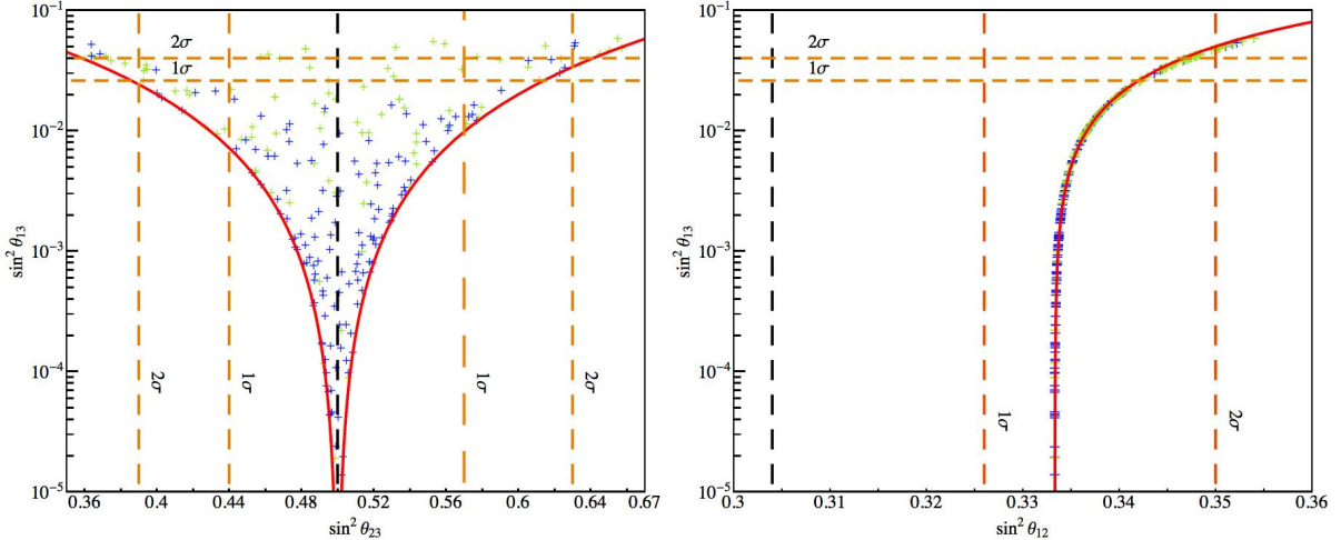
Figure 3: Correlation between \sin^2 \theta_{13} and \sin^2 \theta_{23} (left panel) and \sin^2 \theta_{12} (right panel). Each panel compares the analytical approximations given in eqs. (60) (red lines) with the numerical results. The green and blue points correspond to the IH and NH neutrino spectrum respectively. For the analytical expressions of \sin^2 \theta_{23} we have fixed the CP-Dirac phase \delta at 0. In the numerical analysis the ratio v_S/\Lambda \sim w/\Lambda has been taken in the window bounded from the constraints arising by y_\tau and \sin^2 \theta_{12} , that is 0.007 < v_S/\Lambda < 0.23 . The value of \tan \beta spreads between 2 and 50, while all the other free parameters, y , y_1 , y_2 and y_3 , are treated as random numbers with absolute value between 0.1 and 2. The horizontal dashed orange lines corresponds to the bounds at 1 and 2 \sigma level, respectively, for \sin^2 \theta_{13} , the vertical dashed black line corresponds to the central values of \sin^2 \theta_{23} and \sin^2 \theta_{12} while the vertical dashed orange lines to their bounds at 1 and 2 \sigma level, respectively. The plots are cut in correspondence of the 3 \sigma level bound for \sin^2 \theta_{13} , \sin^2 \theta_{23} , \sin^2 \theta_{12} .
