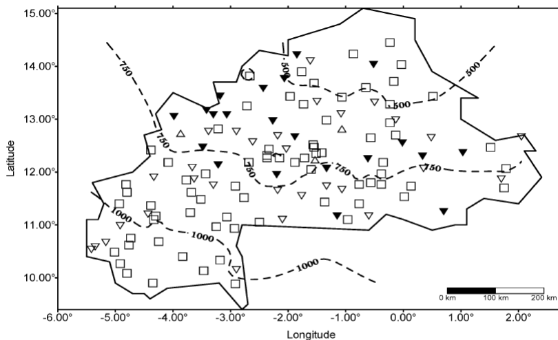
Figure 3. Trends in the iNDVI/RR ratio during the growing season (May–October) for 128 stations in Burkina Faso (1982–1999). ▼, strong negative change; ▽, weak negative change; □, stable; △, weak positive change.
