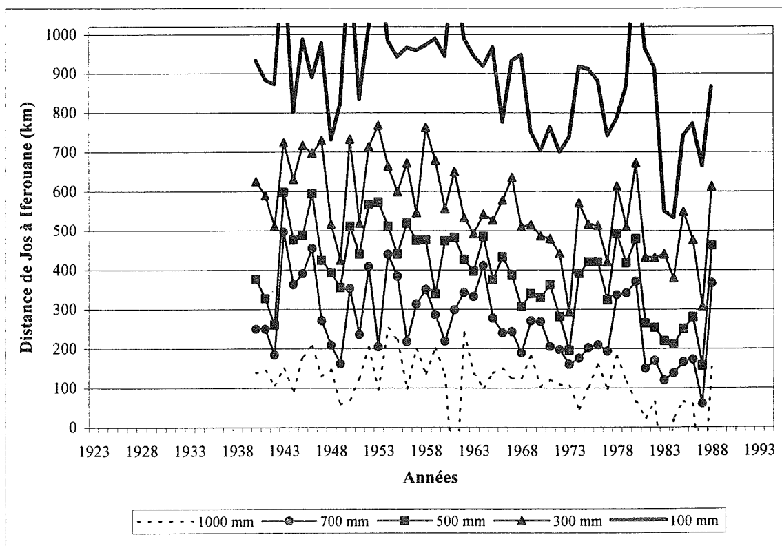
Fig.III.10 - Transect pluviométrique spatio-temporel de Jos à Iferouane de 1940 à 1988. Rainfall profile in space and time from Jos to Iferouane for the 1940–1988 period.
