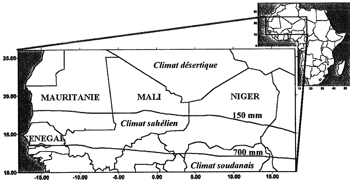
Fig.I.1. - Zone d'étude. Study area.
