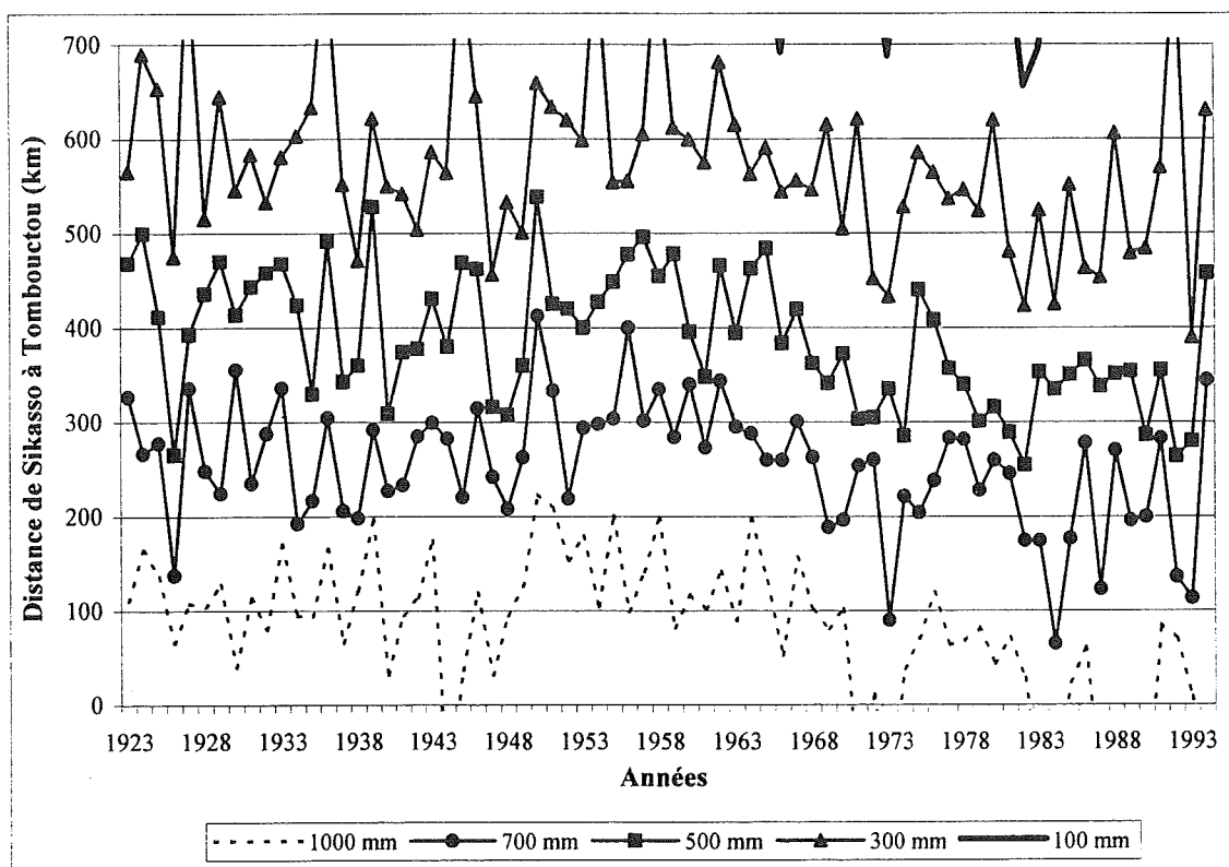
Fig.III.8 - Transect pluviométrique spatio-temporel de Sikasso à Tombouctou de 1923 à 1994. Rainfall profile in space and time from Sikasso to Tombouctou for the 1923–1994 period.
