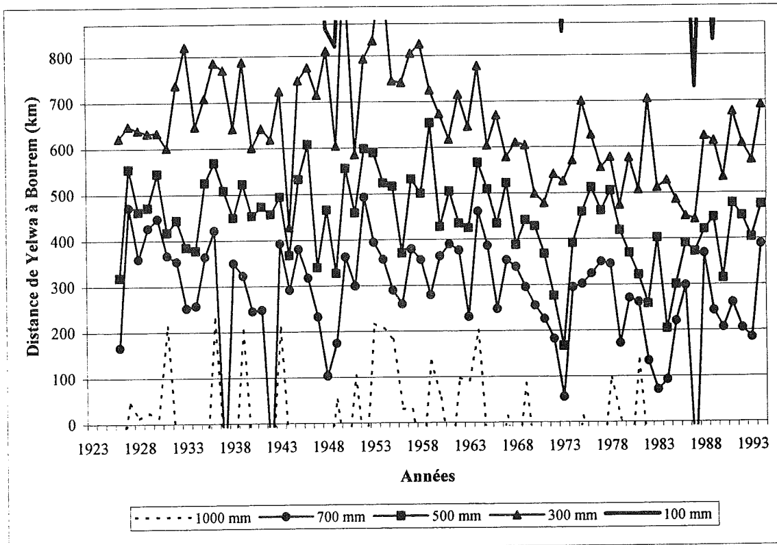
Fig.III.9 - Transect pluviométrique spatio-temporel de Yelwa à Bourem de 1926 à 1994. Rainfall profile in space and time from Yelwa to Bourem for the 1926–1994 period.
