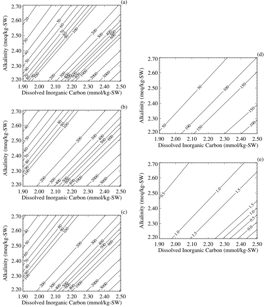
Figure 2.3: Variations of p_{\text{CO}_2} (contours in \mu\text{atm} ) in cold surface waters ( T = 274.16 \text{ K} and S = 35 ) as a function of dissolved inorganic carbon and alkalinity, calculated by adopting different approximations for A_T : (a) — using A_T \simeq A_C , i.e., neglecting the contributions from \text{B}(\text{OH})_4^- , \text{OH}^-_{\text{sWS}} and \text{H}^+_{\text{sWS}} to A_T , defined by (2.49); (b) — using A_T \simeq A_{\text{CB}} , i.e., neglecting only the contributions from \text{OH}^-_{\text{sWS}} and \text{H}^+_{\text{sWS}} ; (c) — using the complete definition (2.49); (d) = (b) - (a); (e) = (c) - (b).
