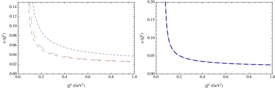
Figure 1: The running of the coupling constant. Left: The short dashed curve corresponds to the LO solution, the medium dashed curve to NLO solution and the long dashed curve to the NNLO solution ( \Lambda = 250 MeV). Right: The solid curve represents the NLO solution with \Lambda = 250 MeV, while the long dashed curve the NNLO solution with a value of \Lambda = 235 MeV.
