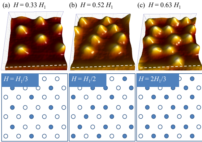
FIG. 2: Upper row: scanning Hall probe microscopy images obtained for sample A at the sample's edge as indicated by the dashed box in Fig. 1 after cooling down to T = 6.9 K in presence of a field H = 0.33H_1 (a), H = 0.52H_1 (b), and H = 0.63H_1 (c). The dashed line shows the sample's edge. Lower row: schematic representation of the expected vortex patterns according to Ref. [21]. Here the open (filled) circles represent empty (occupied) pinning sites.
