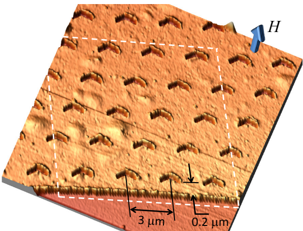
FIG. 1: Atomic force microscopy image of Sample A. The scanning Hall microscopy images of this work have been taken in a region of the sample with the same size ( 12 \mu\text{m} side) and same antidot distribution as the one delimited by the dashed lines. Notice that the first row of boomerang shaped antidots is only 0.2 \mu\text{m} away from the edge of the film. The arrow indicates the direction of the applied field perpendicular to the plane of the film.
