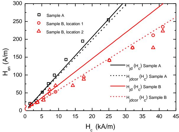
FIG. 4: The obtained experimental data for the first vortex entry field versus H_c(T) obtained by Decker et al. is shown for sample A (square symbols) and for two locations at the border for sample B (circular and triangular symbols). The theoretical curves obtained from Eq.5 for sample A and B with C = \frac{3\sqrt{6}}{4} are shown by the full black and red lines, respectively. The black and red dashed lines take into account the effect of the pattern induced enhancement of the screening current density for sample A and B, respectively.
