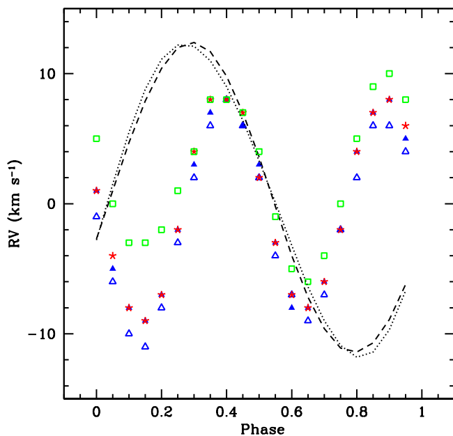
Fig. 12. The difference between RV measurements made on the perturbed and unperturbed spectra \delta(RV) = (RV)_p - (RV)_u for He I \lambda 4921 (open triangles), He I \lambda 5875 (filled-in triangles), Si III \lambda 4552 (stars) and H \beta (squares). Also shown is the shape of the perturbed (dash) and unperturbed (dots) RV curves for He I \lambda 5875 after down-scaling by a factor of 10 for illustration purposes. The perturbation leads to a RV curve corresponding to a more eccentric orbit than the actual orbit.
