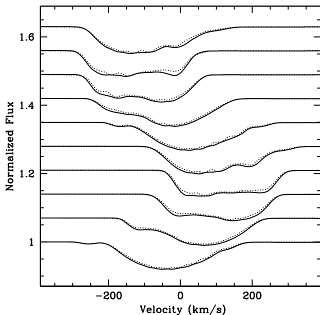
Fig. 14. The Si III \lambda 4552 line profiles computed with ComBiSpeC compared with the line profiles computed with the TIDES code (dots). In this TIDES calculation, the computation is performed using Voigt local line profiles. The ComBiSpeC code uses the same velocity field that is computed with TIDES, but the local line profile is obtained from the non-LTE TLUSTY radiative transfer calculation. Only the profiles computed for the primary star are shown here.
