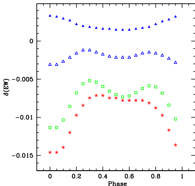
Fig. 7. The difference between equivalent widths measured on the perturbed and unperturbed spectra, \Delta(\text{EW})=[\text{EW}_p-\text{EW}_u]/\text{EW}_u , of the primary star in Spica showing that the effects are \leq 1.5\% , and thus indicating that the interaction effects have a negligible impact on the spectral classification. Negative residuals indicate that the absorption in the perturbed profiles is weaker than in the unperturbed profiles. The different symbols correspond to: He I \lambda 4921 (open triangles), He I \lambda 5875 (filled-in triangles), Si III \lambda 4552 (stars) and H \beta (squares).
