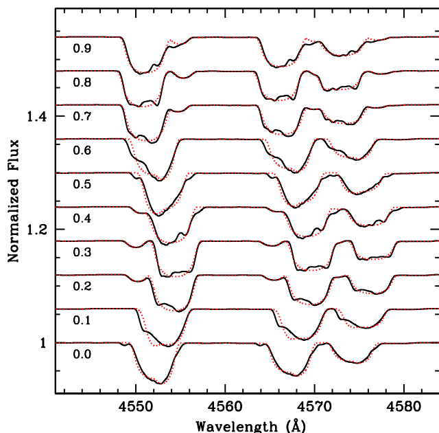
Fig. 9. The synthetic primary + secondary combined spectra of the Si III triplet are stacked in order of increasing orbital phase ( \phi=0 corresponds to periastron). The perturbed spectra are displayed with the dark tracing and the unperturbed spectra with dots. The “bumps” in the primary star’s perturbed profiles are evident as is the difficulty they introduce in properly locating the contribution of the secondary except at \phi \sim 0.3 \pm 0.05 and 0.8 \pm 0.05 when the contribution from the secondary is clearly resolved.
