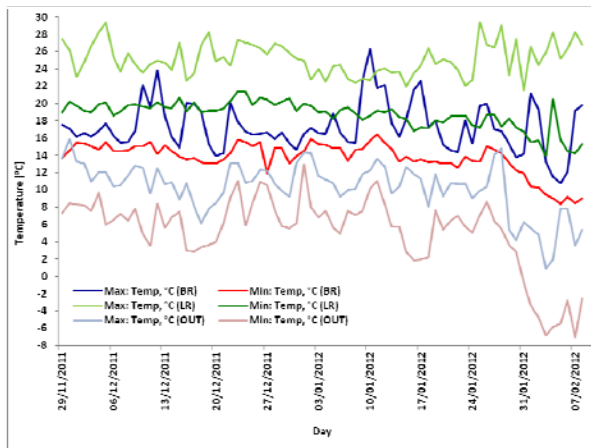
Figure 2a Temperature profile in winter season (House W_8)
