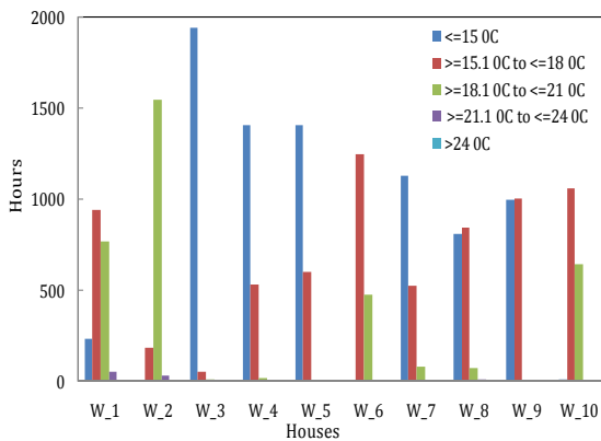
Figure 3a Temperature range and duration of various houses : Bedroom (winter monitoring)
