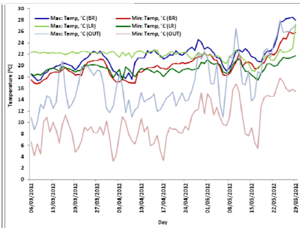
Figure 2b Temperature profile in spring season (House S_1)
