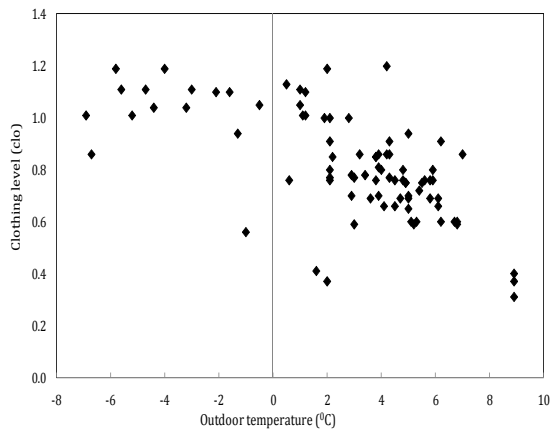
Figure 4a Clothing level against outdoor temperature
