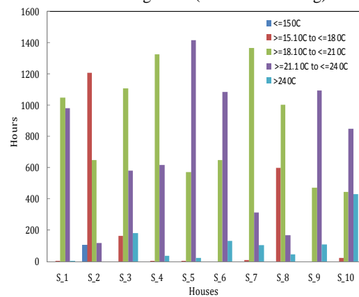
Figure 3d Temperature range and duration of various houses : Living room (spring monitoring)
