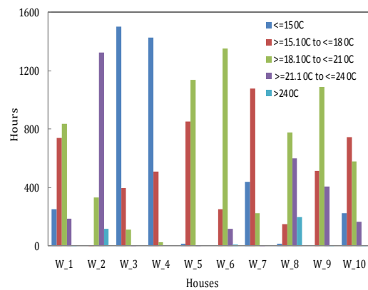
Figure 3b Temperature range and duration of various houses : Living room (winter monitoring)
