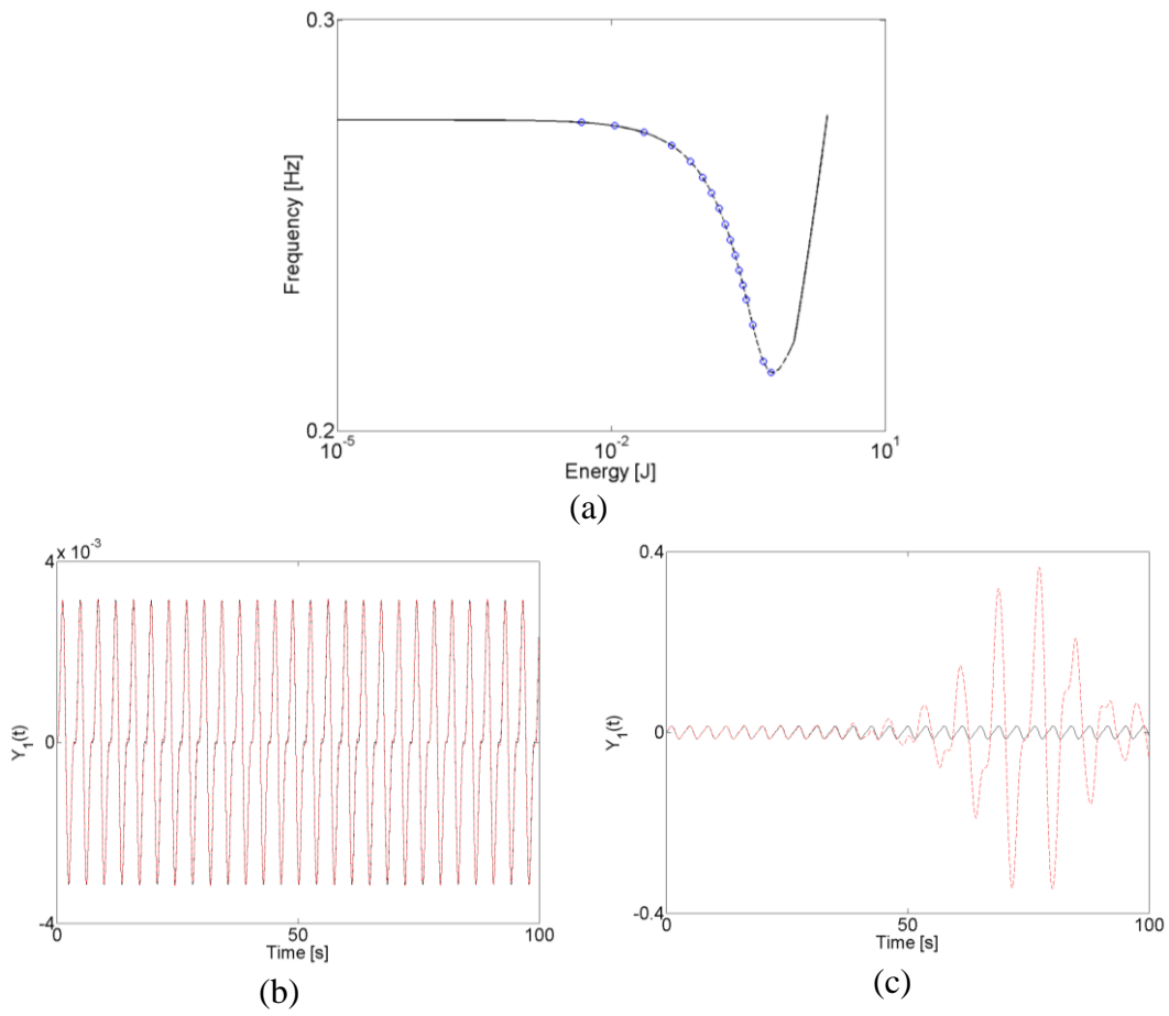
Figure 5. Second NNM. (a) Comparison between the frequency extracted from the invariant manifold (O) and the reference FEP from continuation. The dashed line corresponds to the unstable part of the backbone. (b-c) Slave velocity Y_1 time series reduced on the manifold (black) and for the full-system (red). Perfect matching for low amplitude initial conditions (b). Large discrepancies are observed after 40 seconds.
