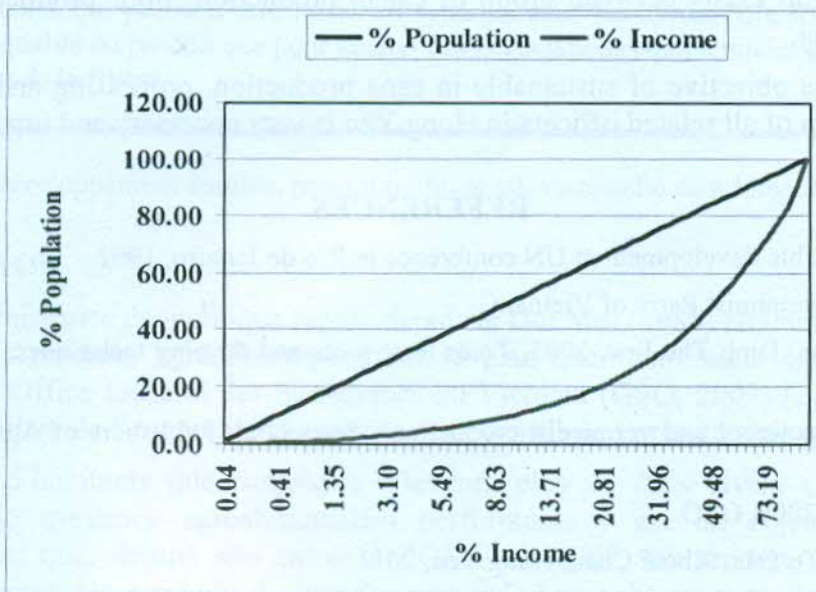
Figure 3: Lorenz curve
