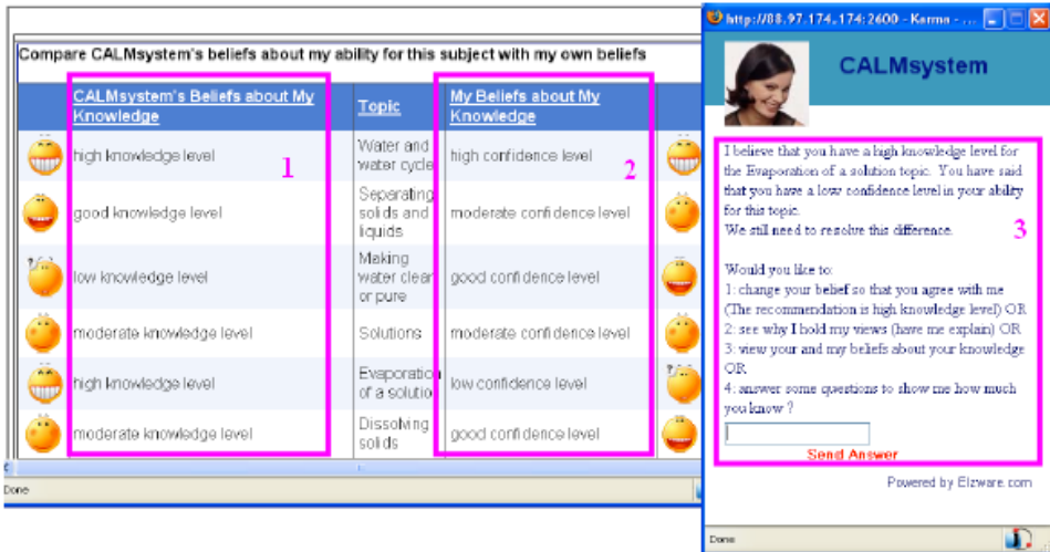
Figure 9.1. Learning Dashboard of the CALM system.
