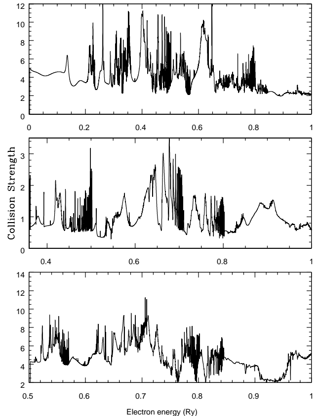
Fig. 6. Collision strengths in JJ-coupling for transitions 3s^23p^2P^o_{1/2} - 3s^23p^2P^o_{3/2} (top panel), 3s^23p^2P^o_{3/2} - 3s3p^2\ ^4P_{3/2} (middle panel), and 3s^23p^2P^o_{3/2} - 3s3p^2\ ^2D_{5/2} (bottom panel).
