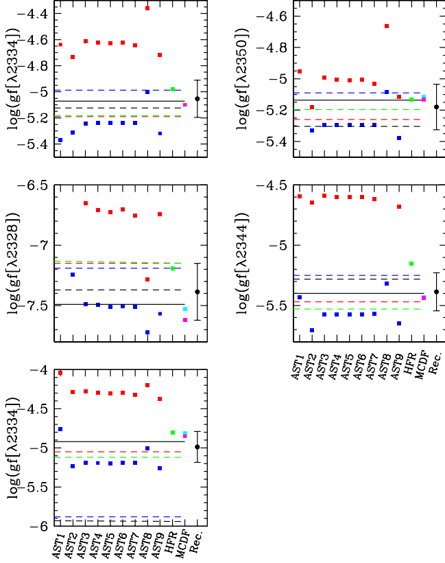
Fig. 4. Evolution of the gf -values for intercombination transition in Si II from our different calculations AST1, ..., AST9 and comparison with experimental values of Calamai et al. (1993). The square points depict our results in the length gauge (blue) and velocity gauge (red). The experimental values are given by the horizontal solid line, with quoted errors given by dashed lines.
