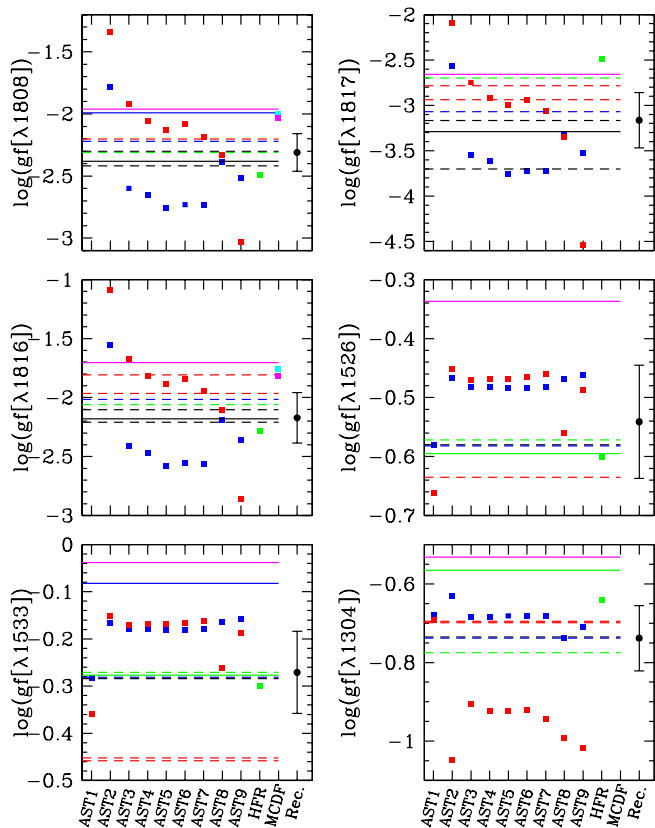
Fig. 2. Evolution of the gf -values for transitions in Si II from our different calculations AST1, ..., AST9 and comparison with previous determinations. The square points depict our results in the length gauge (blue) and velocity gauge (red). The solid horizontal lines depict experimental determinations by Shull, Snow & York (1981) (magenta), Van Buren (1986) (blue), Schectman et al. (1988) (green), Bergeson & Lawler (1993) (black). The dashed lines depict theoretical results of Froese Fischer et al. (2006), (blue), Tayal (2007) (red), Nahar (1988) (green).
