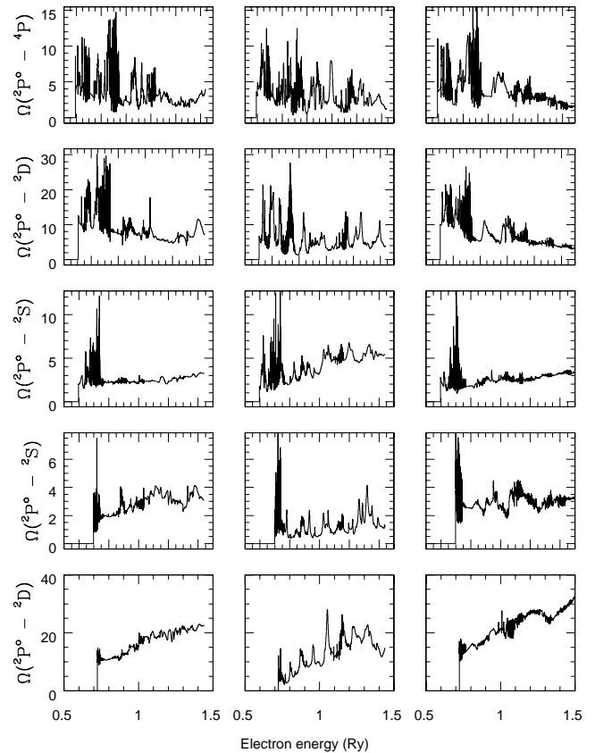
Fig. 5. Comparison of collision strengths in LS coupling for excitations from the ground term to the first five excited terms in Si II computed with approximations AST1 (left panels), AST8 (middle panels), and AST9 (right panels).
