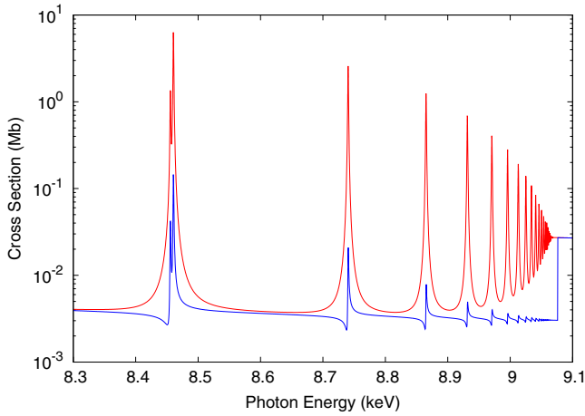
Figure 1. Photoabsorption (upper, red) and photoionization (lower, blue) cross sections of Ne-like Ni near the K edge.
