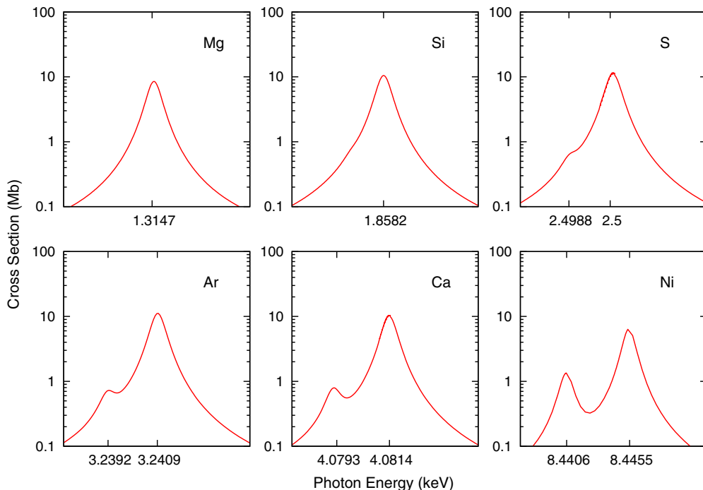
Figure 2. K\beta resonance for Ne-like Mg, Si, S, Ar, Ca, and Ni. Data from the first five ions come from Witthoef et al. (2009). The second resonance appearing from Ne-like S to Ni is due to photoexcitation to the 1s\ 2s^2\ 2p^6\ 3p\ ^3P_1 level.
