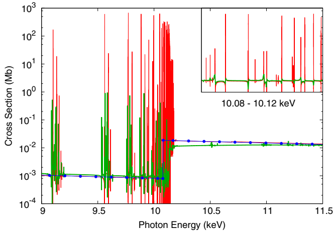
Figure 5. Total photoionization cross section for Li-like Ni from present, R -matrix calculation (thin, red curve), the R -matrix calculation of Nahar (2005; thick, green curve), and Verner & Yakovlev (1995; thin, blue curve with circles). The K\alpha resonances are not visible in this energy range. The background cross sections of Verner & Yakovlev (1995) are in excellent agreement with the present work. Inset: close-up of cross sections between 10.08 and 10.12 keV; range of cross sections is from 10^{-4} to 10^3 . In the inset only, the Nahar (2005) cross sections have been shifted by 8.8 eV to align the resonance positions.
