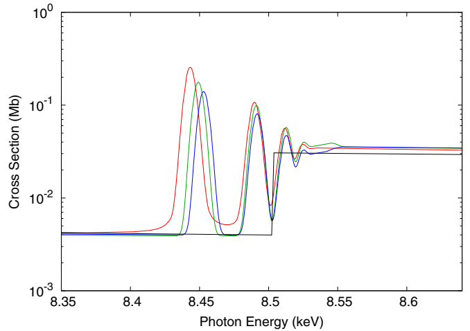
Figure 6. Photoabsorption cross section for Ca-like Ni convolved with a Gaussian having a width of \Delta E/E = 10^{-3} . Based on the height of the resonance feature near 8.45 keV, in order from strongest to weakest, the curves are R -matrix results (red), AUTOSTRUCTURE using target wave functions (green), AUTOSTRUCTURE using parent wave functions (blue), and the background cross section of Verner & Yakovlev (1995; black).
