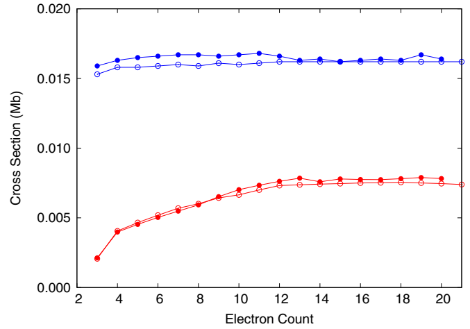
Figure 3. Background cross sections across the isonuclear sequence for the present calculations (filled circles) and Verner & Yakovlev (1995; open circles). The upper two curves (blue) show the cross section above the K edge at 10.9 keV; lower two curves (red) give the cross section below the K edge at 6.8 keV.
