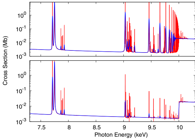
Figure 4. Photoabsorption (top panel) and photoionization (bottom panel) cross sections for Be-like Ni. Red, thin curves show the raw cross section and the blue, thick curves give the convolution with a Gaussian having a width of \Delta E/E = 10^{-4} .
