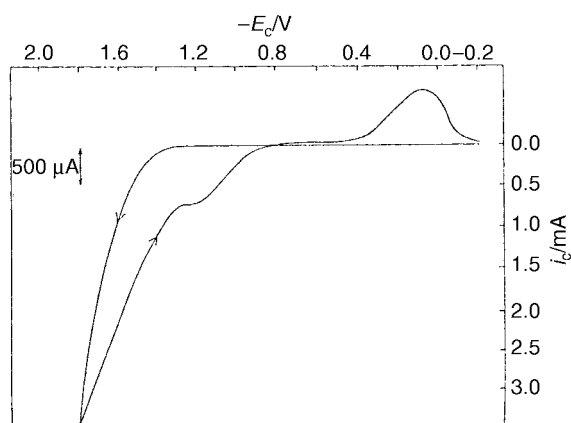
Fig. 6: Cyclic voltammetry recorded on a PE/CB electrode dipped in a \text{GdCl}_3 (0.1 M) solution in FA.
