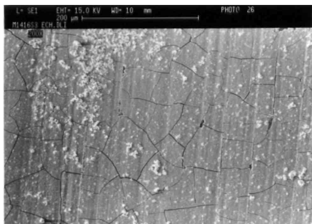
Fig. 7: Micrograph (magnification: 200\times ) of the Gd/Co alloy deposited onto a PE/CB cathode.
