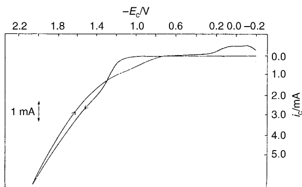
Fig. 6: Cyclic voltammetry recorded on a PE/CB electrode dipped in a \text{GdCl}_3 (0.1 M) solution in FA.
