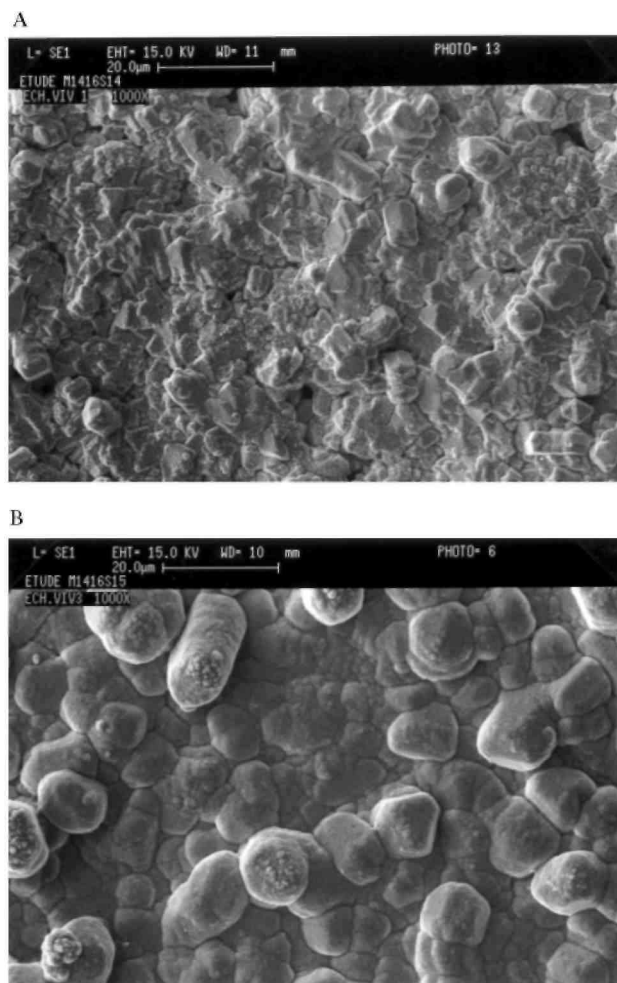
Fig. 2: Micrographs (mag. 1000 \times ) showing the microstructures of (A) Ni coating on Cu/PEDOT/PC, and (B) Gd/Co alloy on Ni/Cu/PEDOT/PC.
