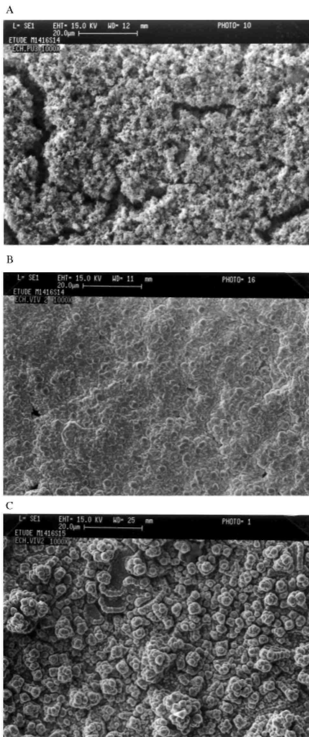
Fig. 1: Micrographs (mag. 1000 ×) showing the micro structures of (A) PEDOT chemically synthesised and sprayed onto a PC plate, (B) Cu thin layer deposited on PEDOT/PC, and (C) Gd/Co alloy deposited on Cu/PEDOT/PC.
