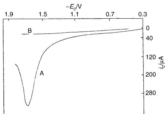
Fig. 10: Cyclic voltammetry recorded on a Gd/Co electrode dipped in acrylonitrile (0.1 M) solution in acetonitrile. (A) First scan, (B) second scan.
