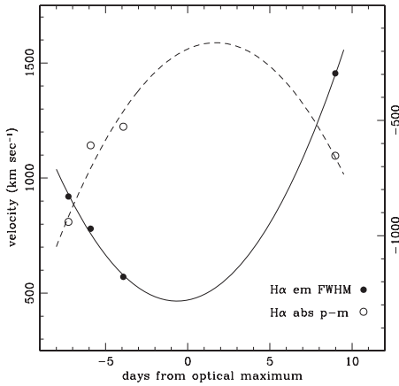
Figure 5. Evolution around maximum brightness of the FWHM of the emission component of H\alpha profile (ordinate scale at left-hand side) and the velocity of the pre-maximum absorption system (ordinate scale at right-hand side). Data from Table 2 and Naito & Narusawa (2007) for t = -7.3 . The fits are explained in Section 3.5.
