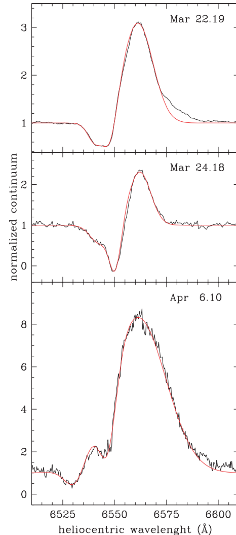
Figure 4. Continuum normalized H\alpha profile of NOph07 on 6 and 4 d before maximum and 9 d past it, at the same time of the low-resolution spectra of Fig. 3. The fit with the emission and absorption components detailed in Table 2 is overplotted.
