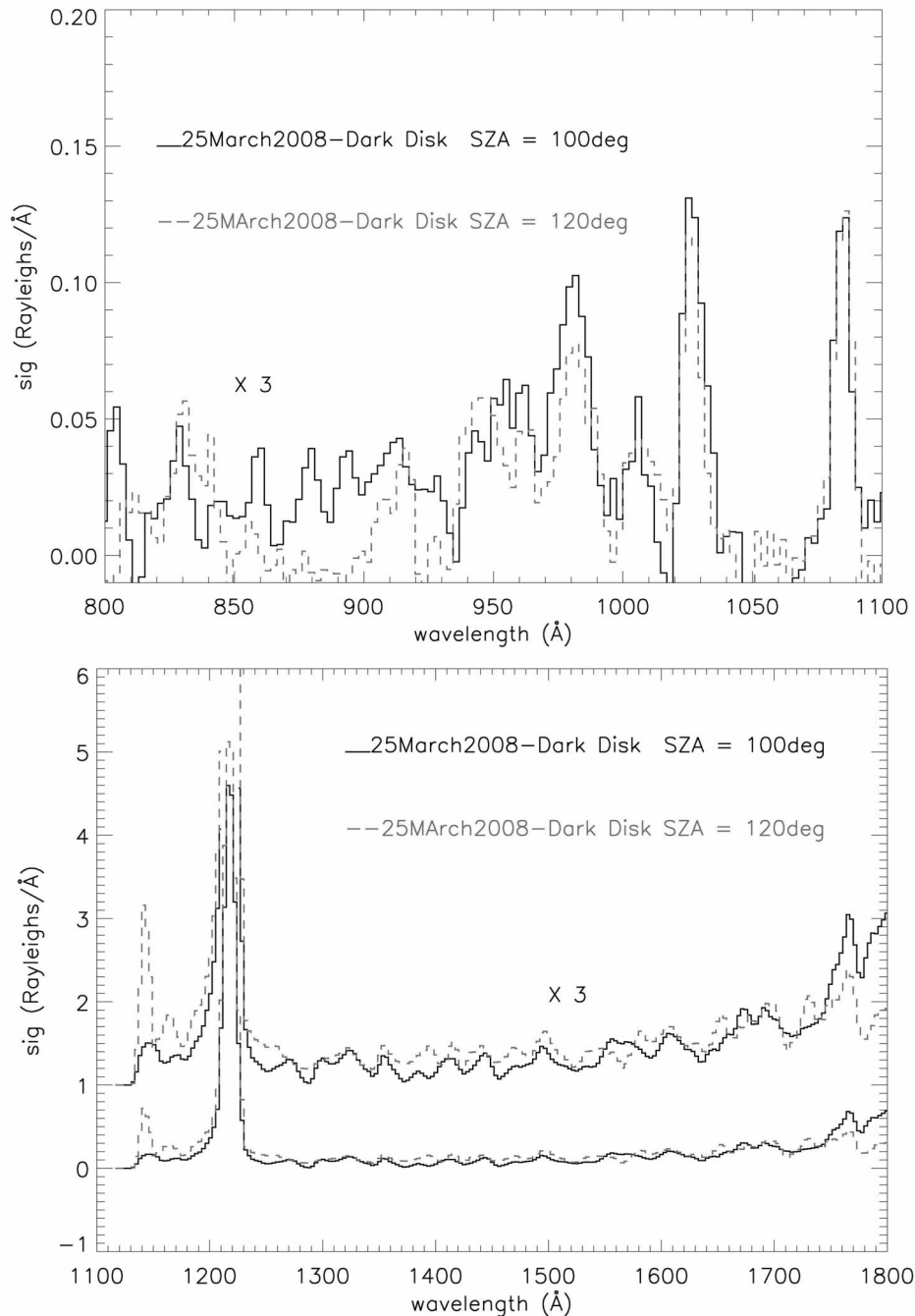
Figure 15. (top) The EUV disk spectrum from 25 March 2008 at 100^\circ ( 90\text{--}110^\circ ) SZA (black) and 120^\circ ( 110\text{--}130^\circ ) SZA (dash-orange). (bottom) The FUV disk spectrum from 25 March 2008 at 100^\circ SZA (black) and 120^\circ SZA (dash-orange).
