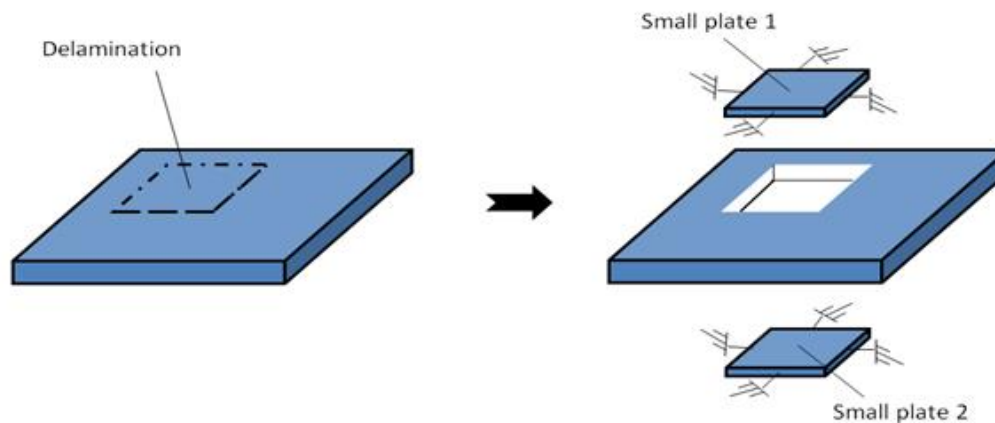
Fig. 2: Local resonance model
