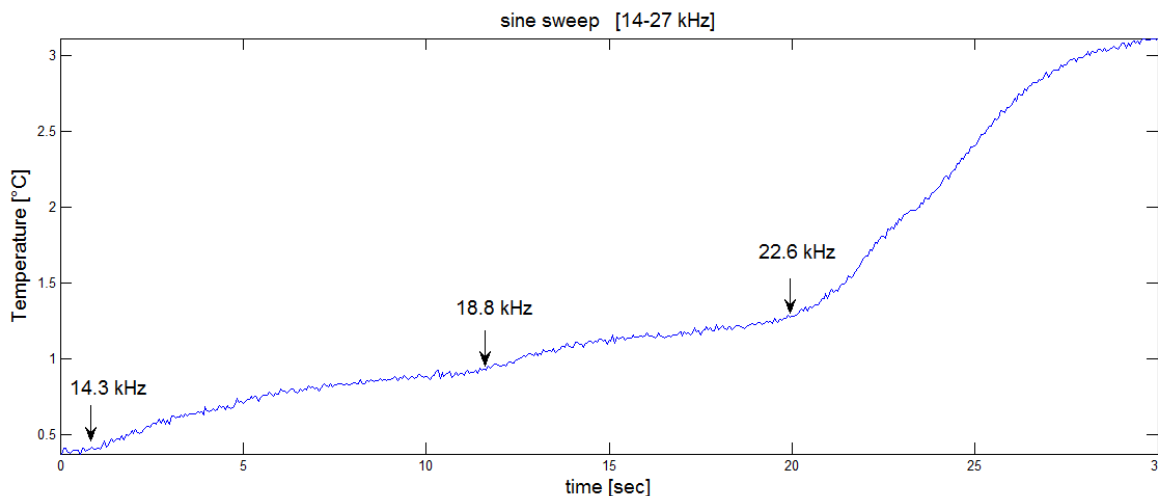
Fig. 6: Temperature increase during linear sine sweep testing
