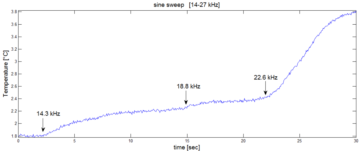
Fig. 7: Temperature increase during logarithmic sine sweep testing
