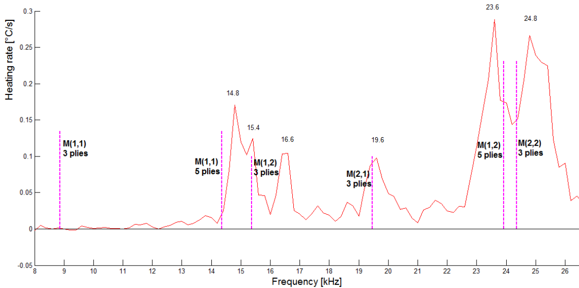
Fig. 5: Heating rate vs. frequency
