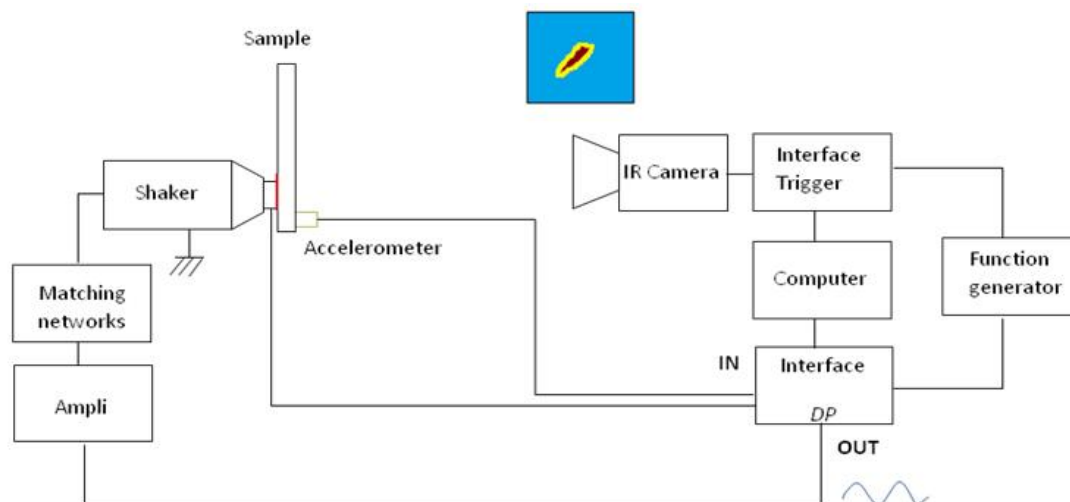
Fig. 1: Test setup
