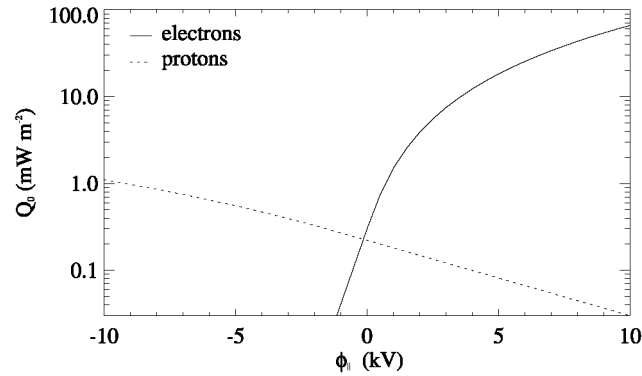
Figure 7: Variation of the precipitating electron and proton energy fluxes ( Q_0(\varphi_{\parallel}) ) with the field-aligned voltage ( \varphi_{\parallel} ), for a plasma sheet "source" population with a number density of 0.5 \text{ cm}^{-3} and proton and electron thermal energies (equal to kT ) of 5 and 0.5 keV, respectively. A positive voltage implies an upward directed electric field. The solid line shows the electron energy flux, while the dashed line shows the proton energy flux.
