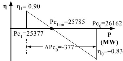
Figure 8-9. Preventive SIME-based stabilization procedure of a relatively « mild » contingency. Conditions of figures 1, 2. Adapted from (Ruiz-Vega, 2002)
