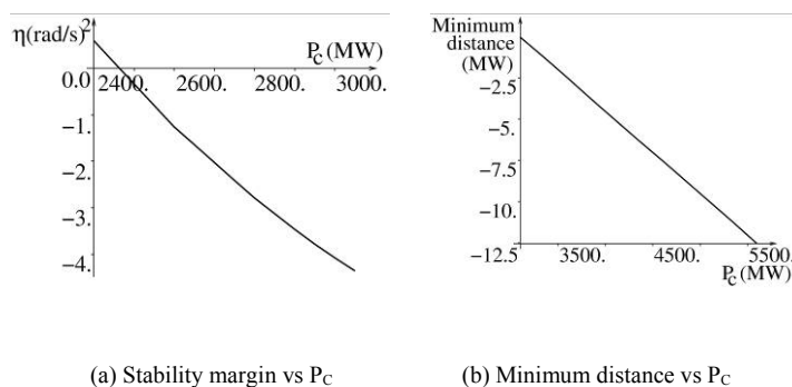
Figure 8-5. Typical variations of the standard stability margin and of its surrogate with P_c . Adapted from (Ruiz-Vega, 2002)
