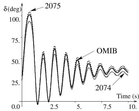
Figure 8-7. Comparison of the swing curves of the OMIB and the critical machines (Nrs 2075 and 2074) of the stable case simulated on the EPRI 627-machine system. Adapted from (Ruiz-Vega, 2002)
