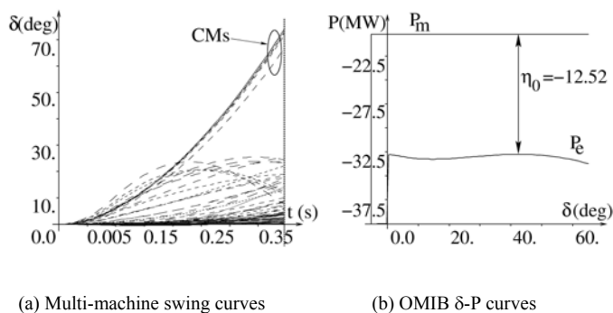
Figure 8-4. Example of a severely stressed case: Clearing time = 95 ms; PC = 5600 MW. Adapted from (Ruiz-Vega, 2002)
