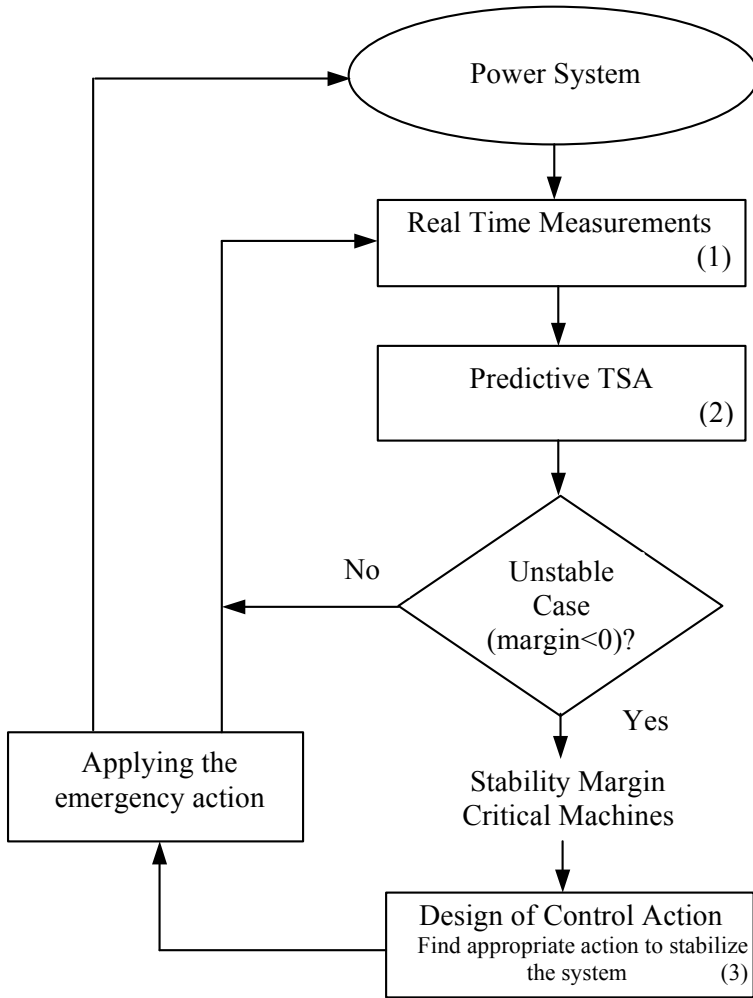
Figure 8-13. Closed-loop transient stability emergency control: general framework. Taken from (Pavella et al., 2000)
