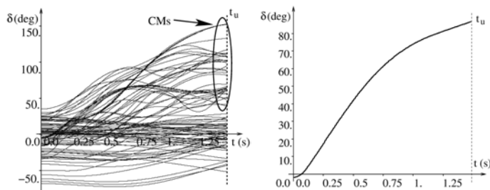
Unstable case. Critical machines power P_C = 26,638 . MW. t_u = 1.48 s.
