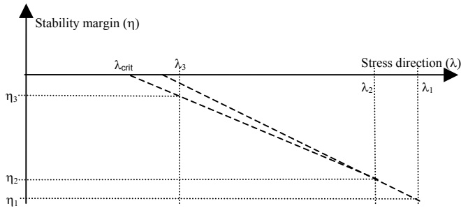
Figure 8-18. Acceleration of limit search by SIME.
