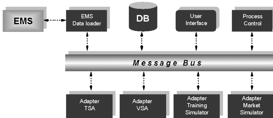
Figure 8-11. OMASES architecture and application functions. Taken from (Cirio et al., 2005)
