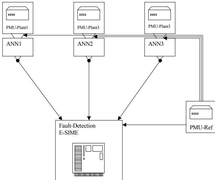
Figure 8-14. Distributed rotor angle estimation and procedure using one PMU device and one artificial neural network per monitored power plant and one reference PMU
