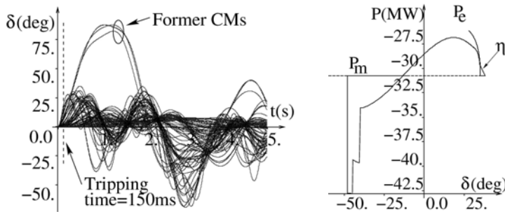
(a) Multi-machine swing curves (b) \delta -P OMIB Curves. P_{c_7} = 2415 MW
