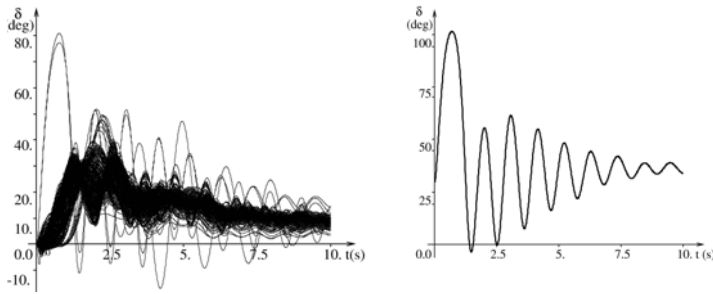
(c) Multi-machine swing curves
