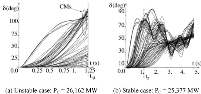
Figure 8-1. Multi-machine swing curves. Critical clearing time: 69 ms; clearing time: 95 ms. Adapted from (Ruiz-Vega, 2002)
