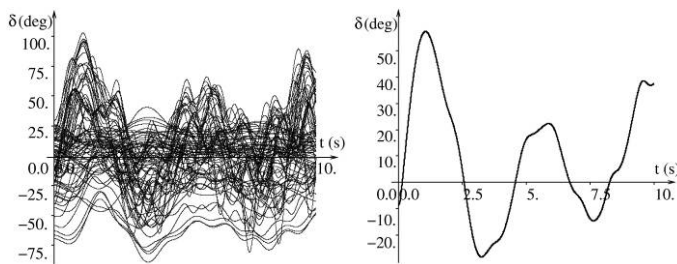
Stable case. Critical machines power P_C = 26,103 . MW
