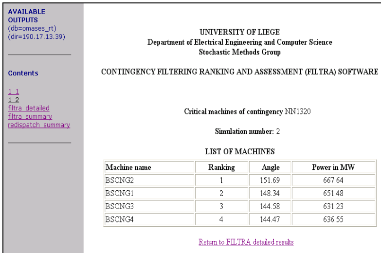
Figure 8-12. FILTRA results and critical machines of Brindisi power station. Taken from (Cirio et al., 2005)
