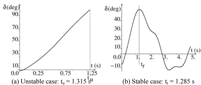
Figure 8-2. Corresponding OMIB swing curves. Adapted from (Ruiz-Vega, 2002)
