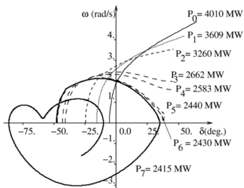
Figure 8-17. OMIB phase plane representation of the 7 simulations described in Table 8-4. Two generators tripped if the contingency actually occurs. Adapted from (Ruiz-Vega, 2002)
