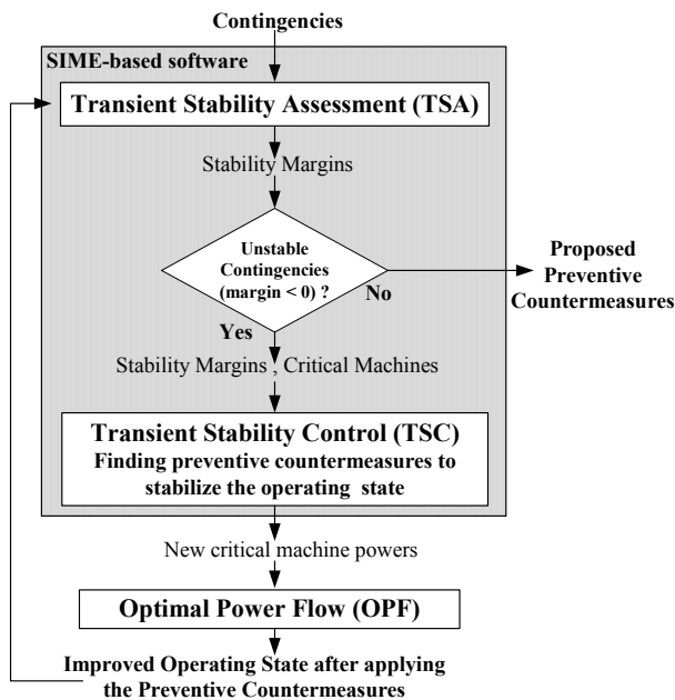
Figure 8-10. Transient stability-constrained OPF (sequential approach). Adapted from (Ruiz-Vega, 2002)
