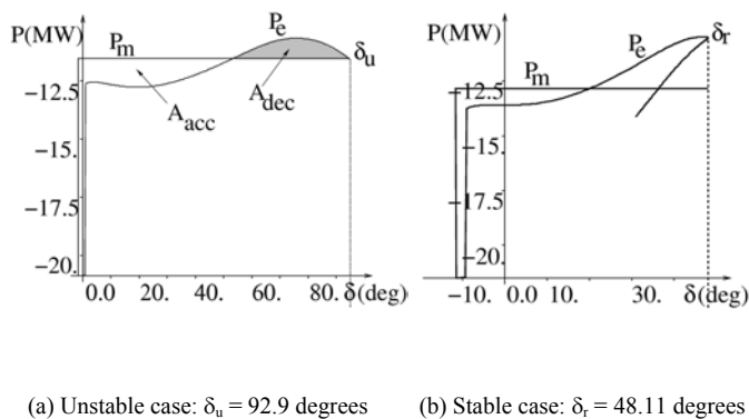
Figure 8-3. Corresponding OMIB \delta -P curves. Adapted from (Ruiz-Vega, 2002)
