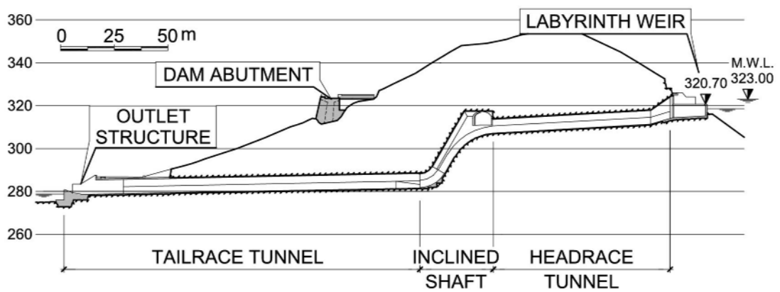
Figure 2. General layout and longitudinal section of the new spillway at the Esch-sur-Sûre dam.
