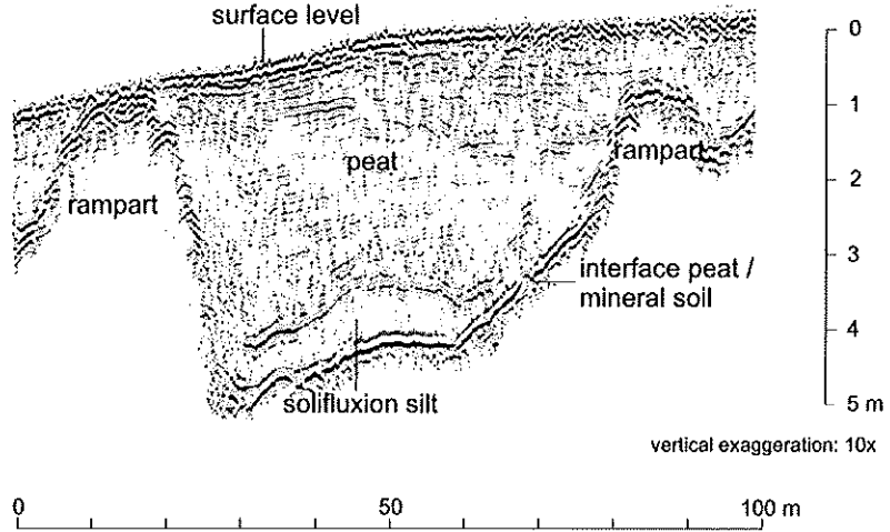
Fig. 2. Vertical section through a lithalsa remnant. The depression was filled in with peat underlain by a solifluxion deposit from the rampart, identified on this radar profile but not present in all instances.
