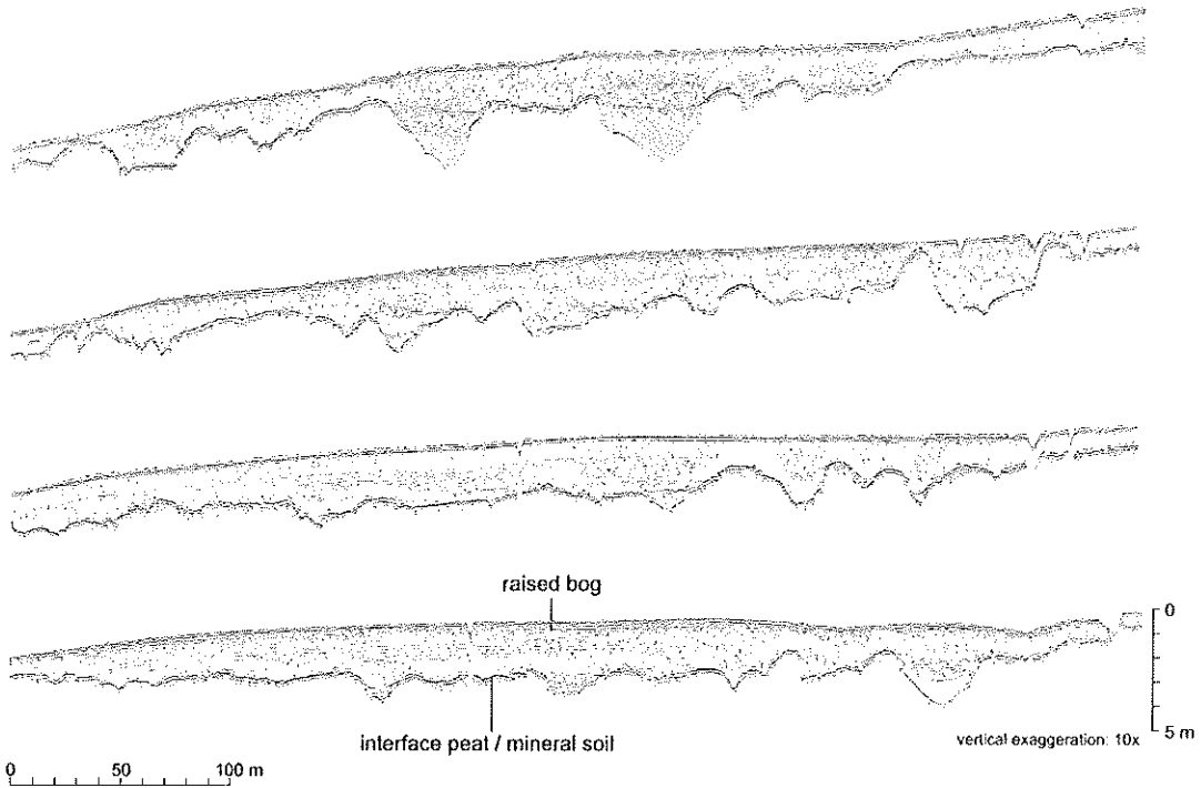
Fig. 4. Subsurface and surface topography in an area of densely grouped lithalsa remnants. The peat formation developed into a raised bog. Successive parallel profiles at 50 m intervals.
