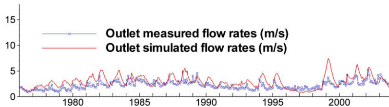
Fig. 7. Transient calibration of surface flow rates for the Kanne gauging station (outlet).
