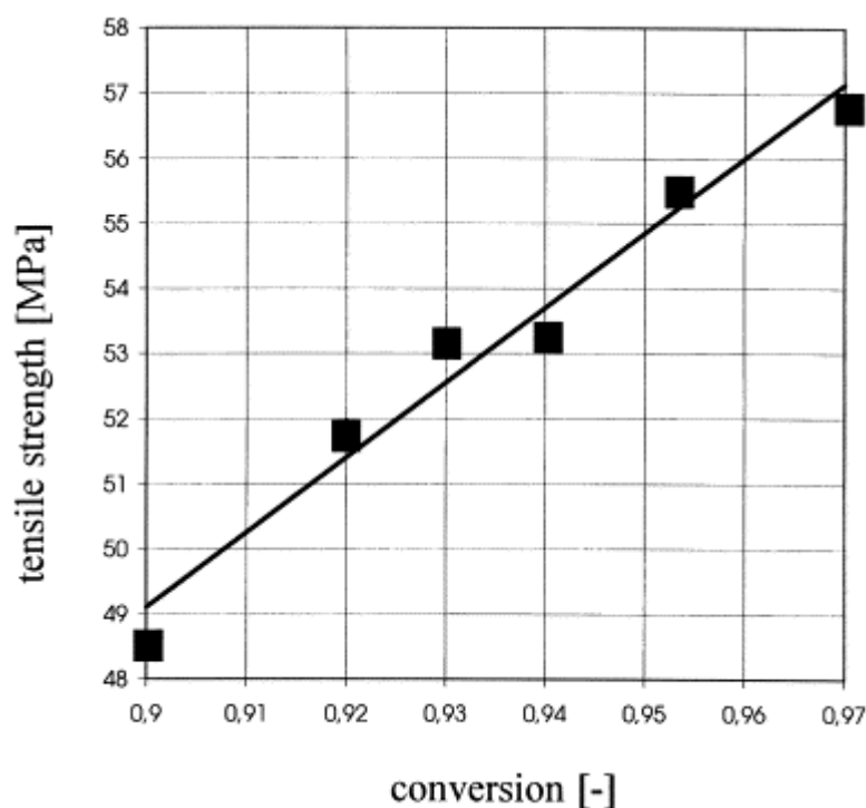
Fig. 6. Tensile strength as a function of reached degree of conversion for poly-L-lactide produced in reactive extrusion polymerisation.
