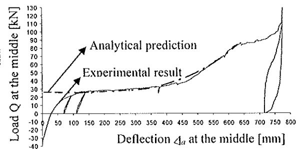
Fig. 7. Comparison analytical prediction vs. experimental results
