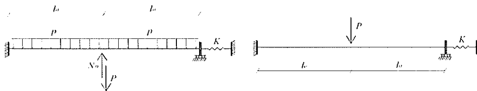
Fig. 11. Considered system with realistic and simplified loadings
