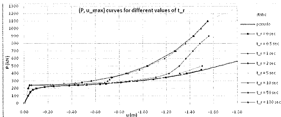
Fig. 13. Maximum dynamic displacement according to the value of the load and its rise time
