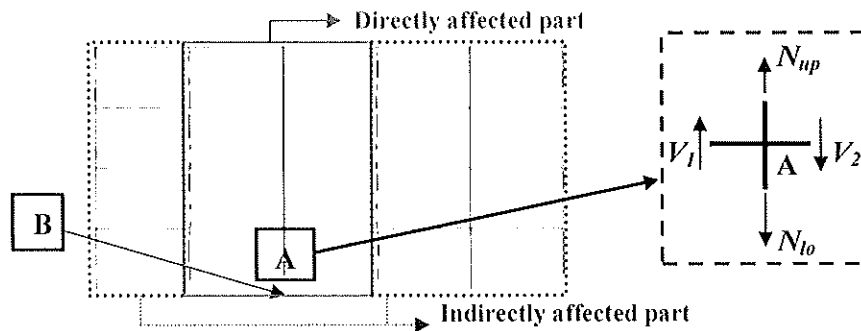
Fig. 1. Representation of a frame losing a column and main definitions
