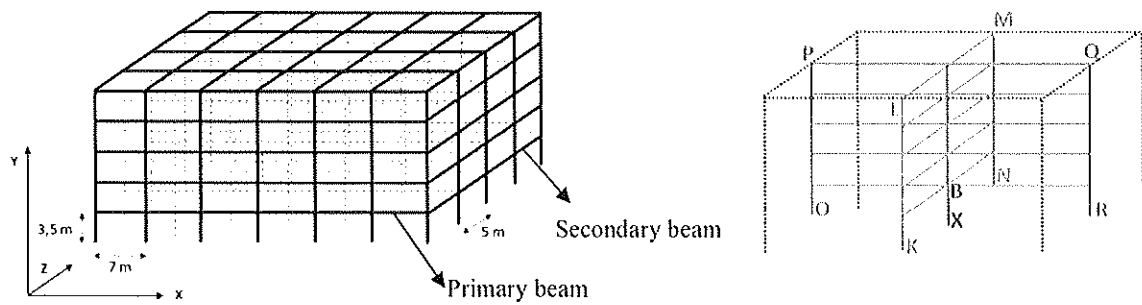
Fig. 8. Investigated 3D structure
