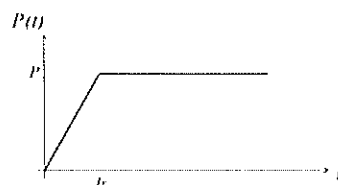
Fig. 12. Time evolution of the applied force P(t)
