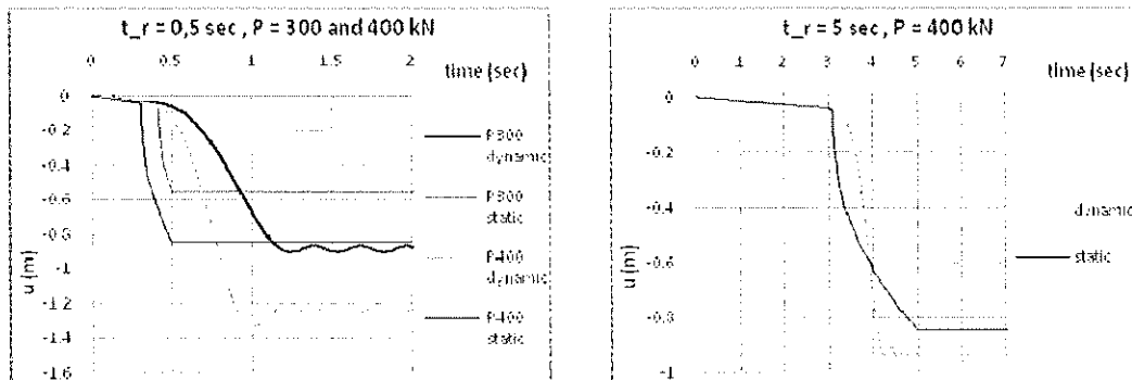
Fig. 14. Examples of the time evolution of the displacement for a response of type 1
