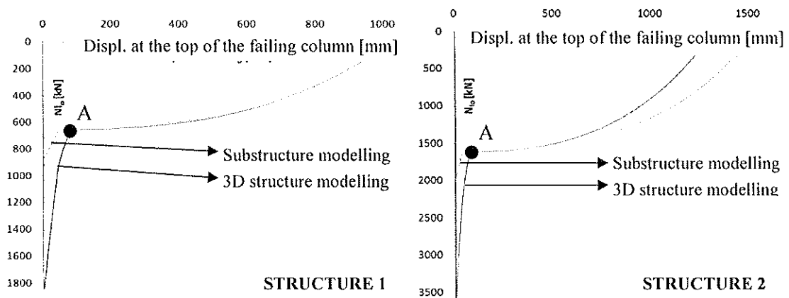
Fig. 10. Comparisons between the results obtained through numerical simulations (i) of the 3D structure and (ii) of the substructure
