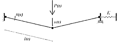
Fig. 17. Considered system and main definitions
