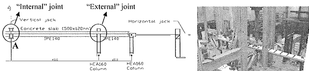
Fig. 4. Tested substructure
