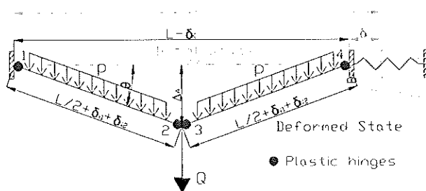
Fig. 6. Substructure to be investigated
