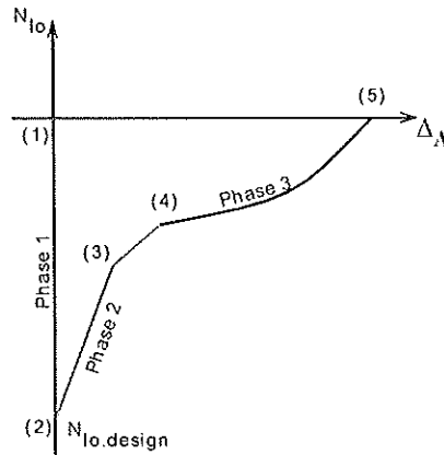
Fig. 2. Evolution of N_{lo} according to the vertical displacement at the top of the loss column
