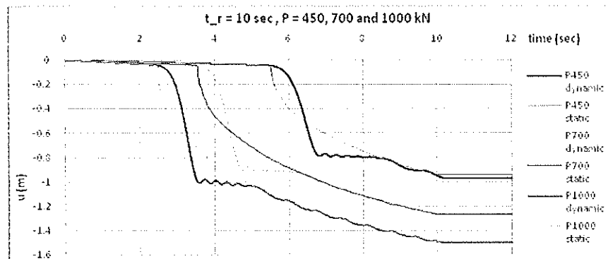
Fig. 15. Examples of the time evolution of the displacement for a response of type 2
