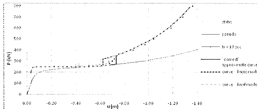
Fig. 13. Example of an approximate dynamic curve
