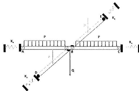
Fig. 9. Substructure extracted from the 3D structure
