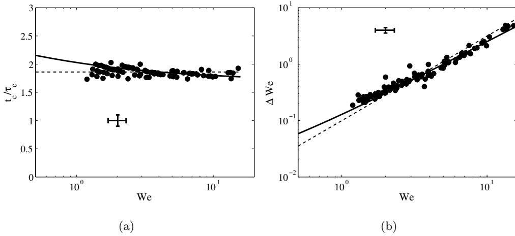
FIGURE 11. (a) Contact time t_c normalized by the capillary time \tau_c = \sqrt{m/\sigma} , and (b) difference in We before and after the bounce as a function of We , for Oh = 0.015 . Dashed lines in (a) and (b) represent fits t_c = 1.86\tau_c and \Delta We = 0.087 We^{3/2} , respectively. Solid lines were deduced by integrating (4.10) with D = 8 \times 10^{-4} \text{ g cm}^{-1} (best fit). The vertical error bar in (a), due to limitations in time resolution, is about \pm 5\% .
