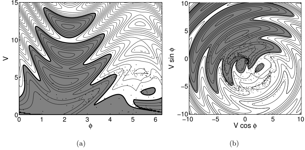
FIGURE 30. Poincaré section at impact of the chaotic attractor at (\Gamma, \omega) = (1.82, 1.21) . (a) Cartesian representation of the (V, \phi) plane, with \Delta E contours superposed (spaced by 5). The shaded area corresponds to a net gain of energy per bounce. (b) Polar representation of the (V, \phi) plane, in which the detailed structure of the attractor is more clear.
