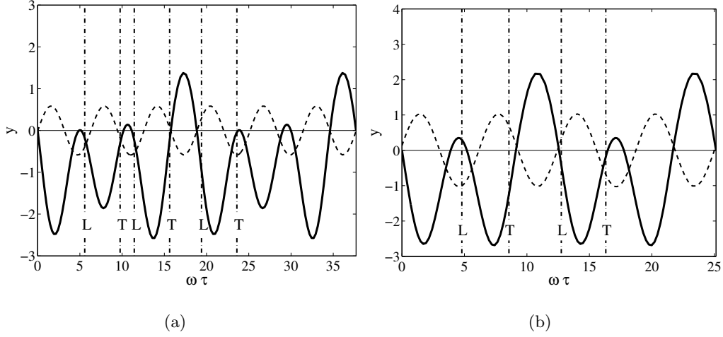
FIGURE 24. (a) Mode (3,3) observed at (\Gamma, \omega) = (0.8545, 1.21) and (b) mode (2,2) observed at (\Gamma, \omega) = (1.5, 1.21) . In both cases, solid lines correspond to trajectories y(t) in the frame of the film, dashed lines correspond to the film motion and dash-dotted lines represent the landing (L) and take-off (T) phases measured experimentally at (\Gamma, \omega) = (0.7, 1.21) and (\Gamma, \omega) = (1.2, 1.21) , respectively.
