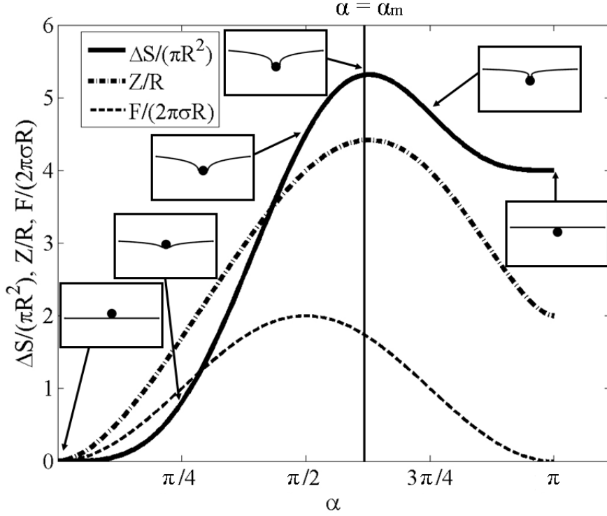
FIGURE 16. Variation of \Delta S/(\pi R^2) , Z/R and F/(2\pi\sigma R) with \alpha , for \beta = A/R = 10 . Insets represent the shape of the film for different values of \alpha , for \beta = 5 .
