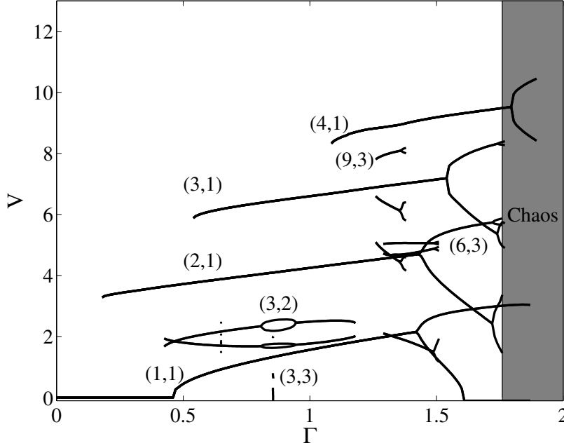
FIGURE 27. Bifurcation diagram for \omega = 1.21 . Dimensionless impact speed V as a function of the dimensionless acceleration \Gamma , as deduced by integrating (4.14). No bouncing is observed below \Gamma = 0.18 . Then, several discrete values of the impact velocity become possible, indicating multi-periodicity. Finally, for \Gamma > 1.76 (shaded area), a few periodic states persist, but chaos prevails.
