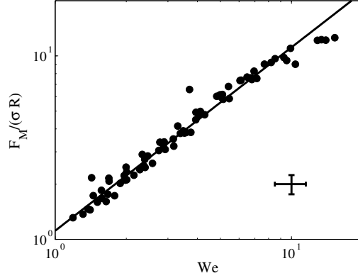
FIGURE 21. Dependence on We of the maximum force F_M applied by the soap film on the droplet, for Oh = 0.015 . The maximum deflection Z is measured experimentally, and F_M is computed according to (3.2) and (3.4). The solid line corresponds to F_M/(\sigma R) = 1.11 We .
