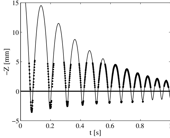
FIGURE 22. Observed (dots) and simulated (solid line) trajectories of a droplet released at We = 15.24 and bouncing on a stationary soap film. Model parameters are m = 2.25 \times 10^{-3} g, k = \frac{8\pi}{7}\sigma = 77 dyn cm ^{-1} and D = 8 \times 10^{-4} g cm ^{-1} (best fit value inferred from figure 11). Experimental data could only be obtained in the apparent field of view, that was partially obscured by the frame of the soap film and also limited from above.
