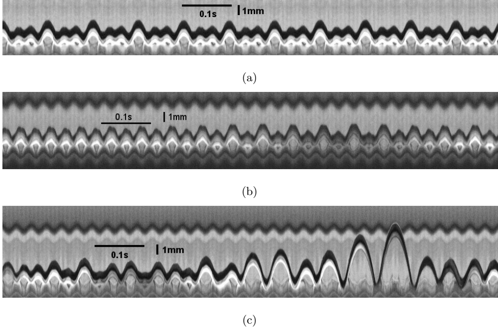
FIGURE 14. Complex bouncing modes. The vertical trajectory of the droplet is displayed as a function of time. (a) A periodic mode (3,3) consists of three successive jumps ( f = 33 Hz, \Gamma = 0.7 g). We = 0.015, 0.074 and 0.3 during the small, the medium and the large jumps, respectively. (b) A period-doubling transition, from mode (1,1) to mode (2,2), observed at f = 33 Hz, \Gamma = 1.2 g. (c) A chaotic bouncing trajectory observed at f = 33 Hz, \Gamma = 1.1 g.
