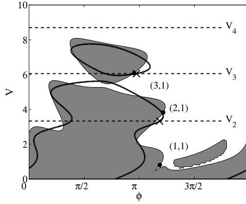
FIGURE 31. Net energy transferred to the drop during impact as a function of the impact velocity V and phase \phi . The forcing parameters are (\Gamma, \omega) = (0.6, 1.21) . In the shaded area, computed numerically by integrating (4.14), the droplet gains energy during impact. The thick line is the leading-order approximation of the shaded area, corresponding to (4.20) and (4.21) deduced for a conservative, unforced system. Dashed lines correspond to velocities prescribed by the compatibility equation (4.19). Modes (m, 1) predicted by numerical simulation are represented by dots and predictions based on the leading-order approach (4.20–4.21) are represented by crosses.
