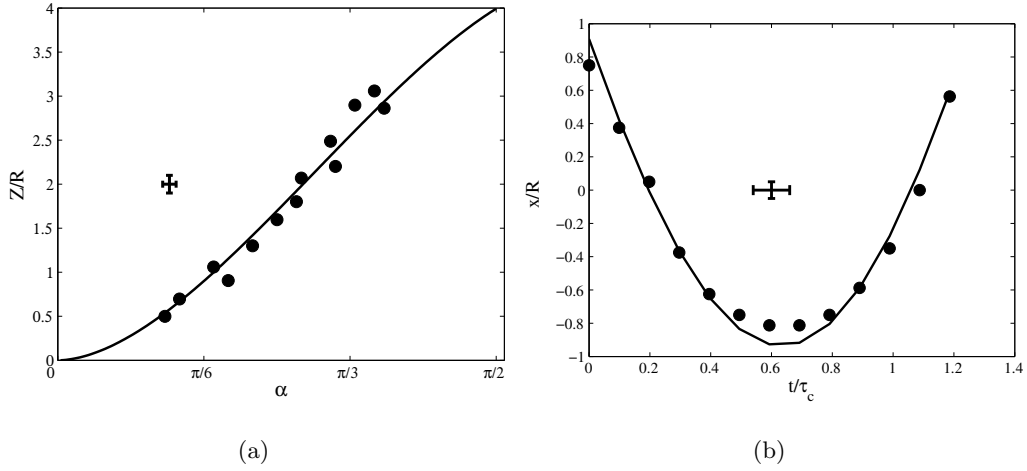
FIGURE 19. (a) Maximum vertical deflection of the film as a function of \alpha , the slope at the matching point. (b) Trajectory of the droplet's center of mass, x . The Weber number is We=9.7 . The solid line represents the trajectory reconstructed from the model (3.6), in which gravity and the force exerted by the soap film are taken into account.
