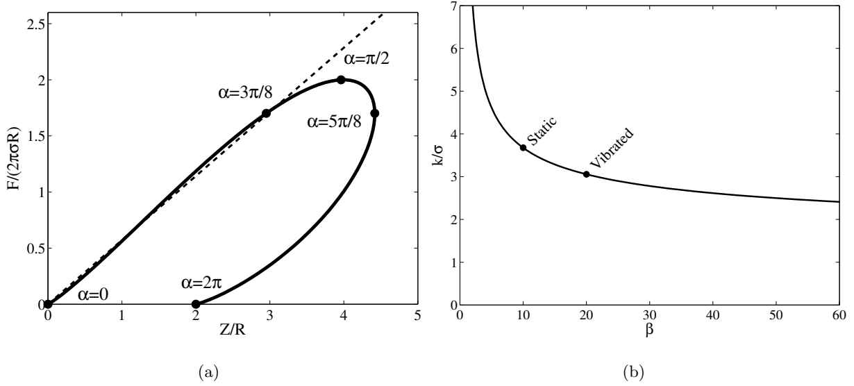
FIGURE 17. (a) Theoretically predicted force–displacement curve for a spherical drop impinging on a soap film. The solid line represents the variation of the force F/(2\pi\sigma R) with respect to the maximum film deflection Z/R for \beta = 10 . The dashed line represents the linear spring approximation (3.5). (b) Stiffness coefficient k/\sigma as a function of \beta . Our static soap film ( \beta = 10 ) has a stiffness k \simeq 8\pi/7\sigma while for the vibrated soap film ( \beta = 20 ), k \simeq 24\pi/25\sigma .
