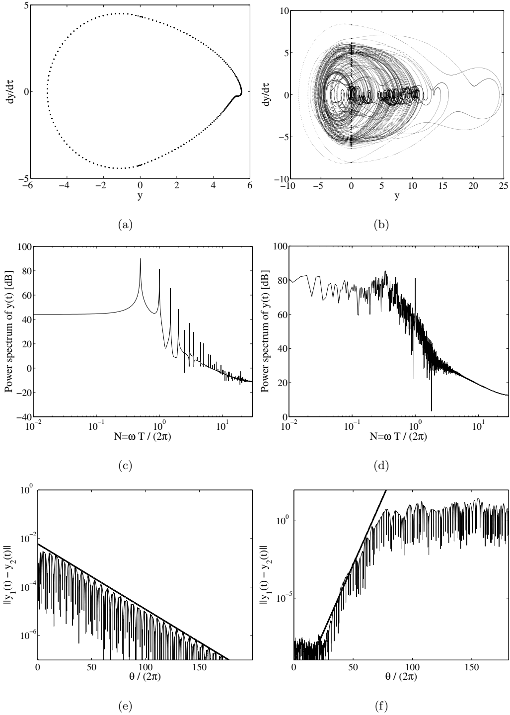
FIGURE 26. Periodic and chaotic solutions for \omega = 1.21 . (a) Limit cycle corresponding to mode (2,1) at \Gamma = 1 . (b) Chaotic attractor at \Gamma = 1.82 . (c) Sparse power spectrum of the limit cycle (a). (d) Full power spectrum of the chaotic attractor (b). Note the peaks at N = \omega T / (2\pi) = 1 , corresponding to the forcing frequency. (e) Distance between points in phase space decreases exponentially for the limit cycle (a), indicating a Lyapunov exponent \lambda \simeq -0.063 . All trajectories collapse onto the limit cycle. (f) For the chaotic attractor (b), the Lyapunov exponent \lambda \simeq 0.4 . Initially neighbouring trajectories diverge exponentially, indicating sensitivity to initial conditions.
