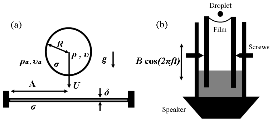
FIGURE 1. Experimental set-up. (a) Without vibration: a droplet strikes a horizontal soap film fixed on a thin ring. (b) With vibration: the soap film is pinned at the end of the inner tube, which is vertically vibrated by a speaker. The arrangement with the outer cylinder ensures a downward curvature of the film, and so stabilizes the bouncing droplet.
