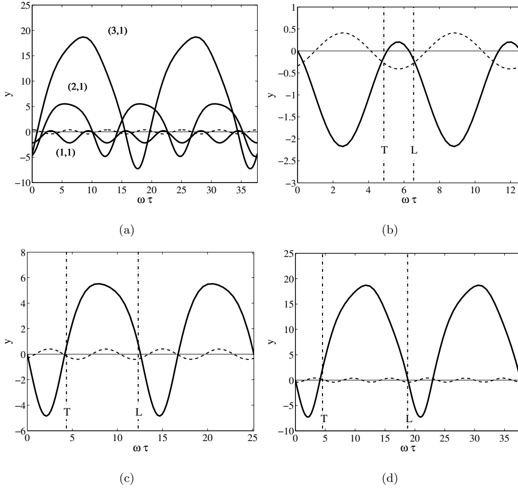
FIGURE 23. Multi-periodicity of bouncing modes at f = 33 Hz ( \omega = 1.21 ) and \Gamma = 0.6 , corresponding to the forcing parameters of the trajectories reported in figure 13. Solid lines correspond to trajectories y(t) computed from (4.14); dashed lines correspond to the film motion; vertical dash-dotted lines represent the landing (L) and take-off (T) phases measured experimentally (figure 13). (a) Modes (1,1), (2,1) and (3,1). (b) Mode (1,1). (c) Mode (2,1). (d) Mode (3,1). Note that the free-fall portion of the trajectory is not a parabola since y(t) is the position of the droplet in a frame that moves with the vibrating soap film.
