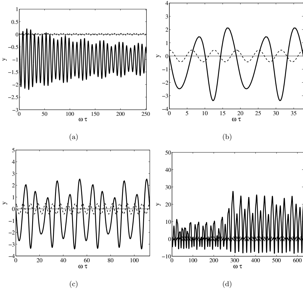
FIGURE 25. Other modes produced by integrating (4.14) for \omega = 1.21 . (a) No bouncing at \Gamma = 0.05 . (b) Mode (3,2) at \Gamma = 0.65 . (c) Mode (9,6) at \Gamma = 0.65 . (d) Chaotic motion at \Gamma = 1.82 . The transition to chaos occurs via a cascade of period-doubling events, each of which transforms a mode (m, n) into a mode (2m, 2n) . The solid line corresponds to the trajectory y(t) in the frame of the ring, and the dashed line to the ring motion.
