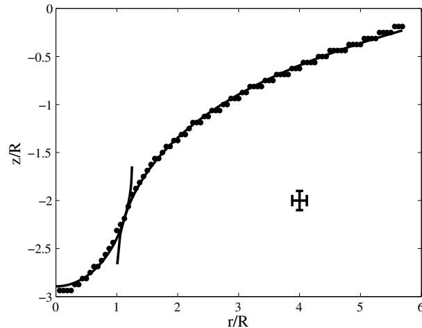
FIGURE 18. Observed shape of the soap film (dots) at We = 9.7 . The thick solid curves represent the ‘sphere plus catenoid’ model: the film has curvature 2/R beneath the drop and zero beyond. calculations become much more complicated, and do not yield further insight into the film dynamics. The relation (3.2) between the angle of matching \alpha and the maximum deformation Z is examined in figure 19(a). Experimental data are gathered from a full cycle of a droplet in a bouncing state. The hysteresis is very weak: the deformation is roughly the same whether the drop is rising or falling, which lends added credibility to our quasi-static description of the soap film.
