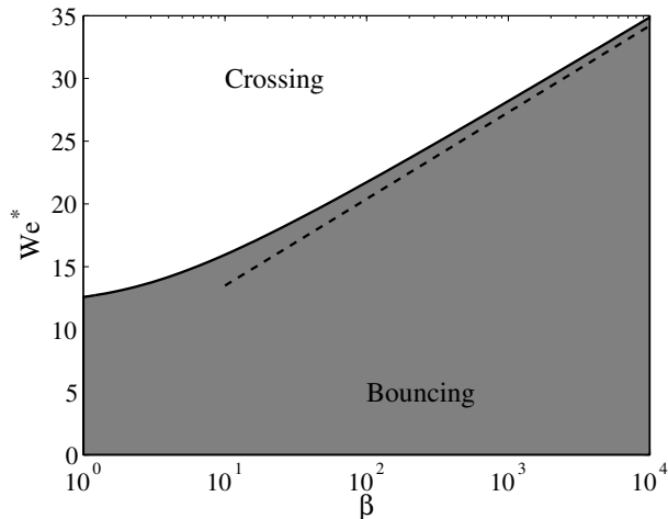
FIGURE 20. Critical Weber number We^* for the bouncing-to-crossing transition, as a function of the ratio \beta = A/R between the soap film and the droplet radii. The solid line corresponds to (3.8), and the dashed line to the asymptotic behavior We^* \sim 4.5 + 3 \ln(2\beta) relevant for \beta \gg 1 .
